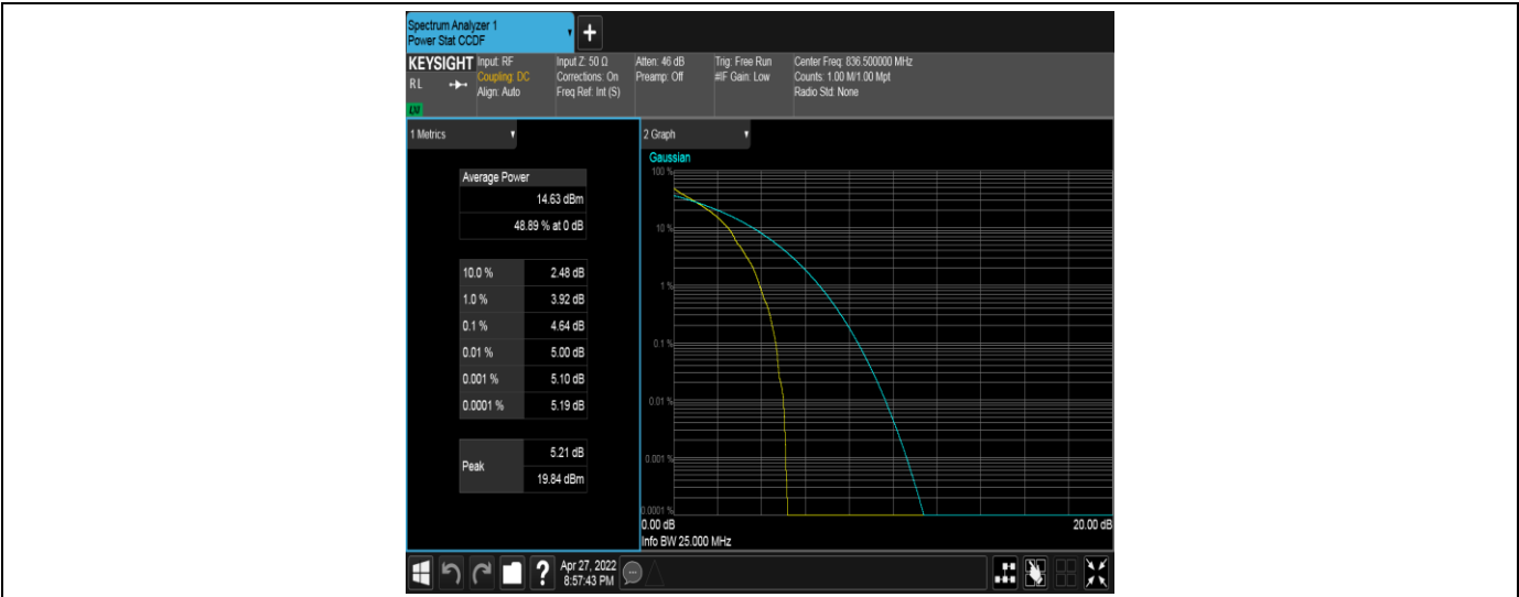
Band5-5MHz-QPSK-20525-25RB#0
