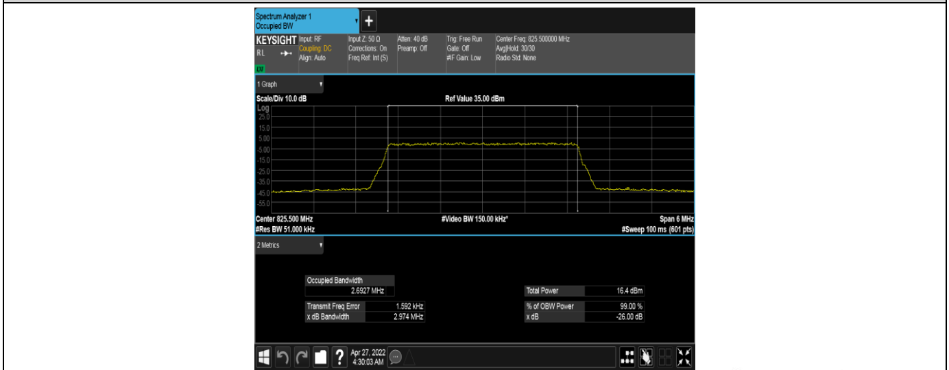
Band5-3MHz-16QAM-20415-15RB#0
