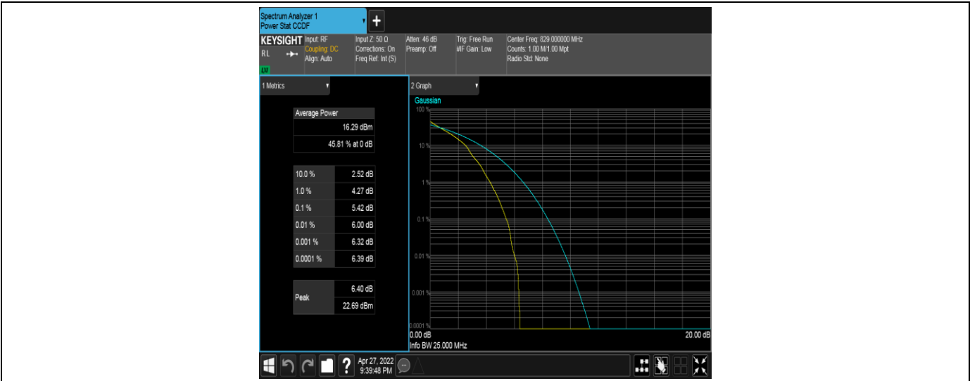
Band5-10MHz-QPSK-20450-50RB#0
