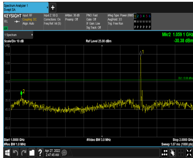
Band4-10MHz-QPSK-20000-1RB#0-Range3:2000~20000MHz
