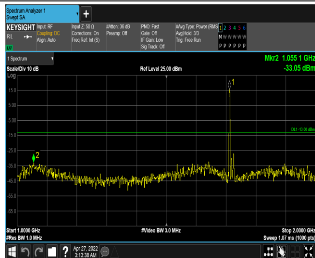
Band4-15MHz-16QAM-20025-1RB#0-Range2:1000~2000MHz
