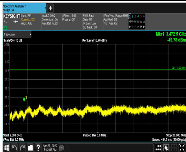
Band4-20MHz-16QAM-20300-1RB#0-Range3:2000~20000MHz
