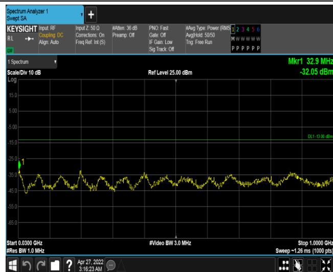
Band4-15MHz-16QAM-20325-1RB#0-Range1:30~1000MHz
