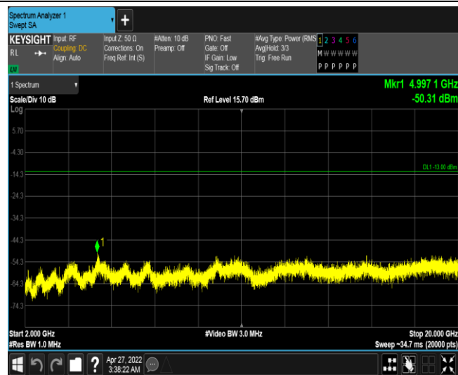
Band4-20MHz-QPSK-20050-1RB#0-Range3:2000~20000MHz
