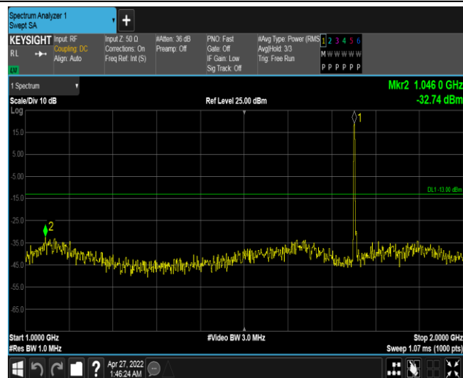
Band4-5MHz-16QAM-20375-1RB#0-Range2:1000~2000MHz
