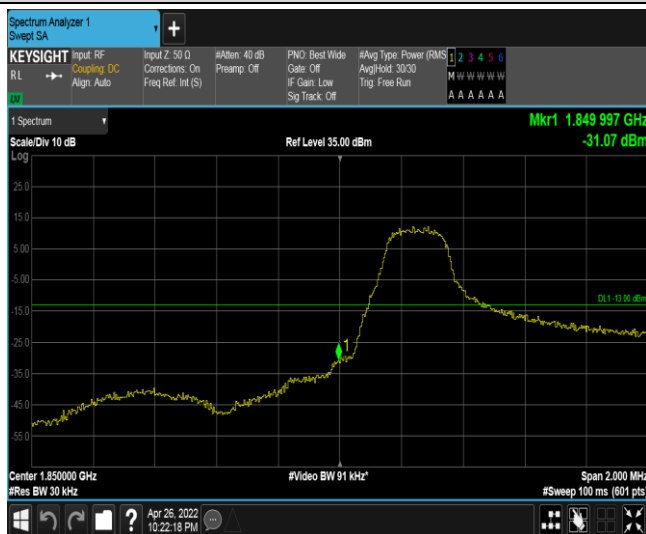
Band2-1.4MHz-QPSK-18607-1RB#5
