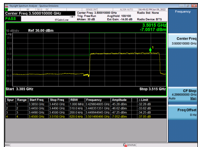
N77(60M)_CP-OFDM_QPSK_Edge_ Outer_Full_Low_CH
