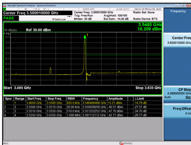
N77(80M)_CP-OFDM_QPSK_Edge_ 1RB_Right_High_CH
