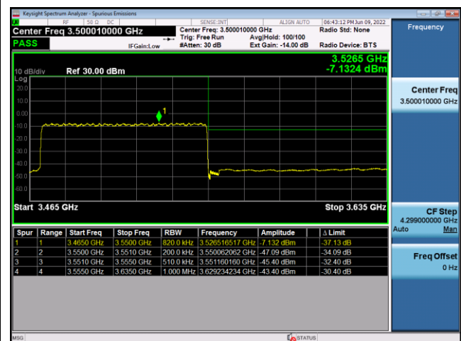
N77(80M)_CP-OFDM_QPSK_Edge_ Outer_Full_High_CH
