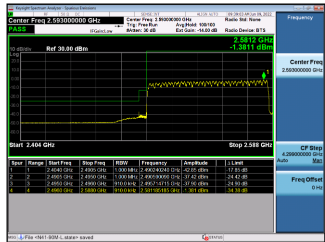
N41(90M)_CP-OFDM_QPSK_Edge_ Outer_Full_Low_CH
