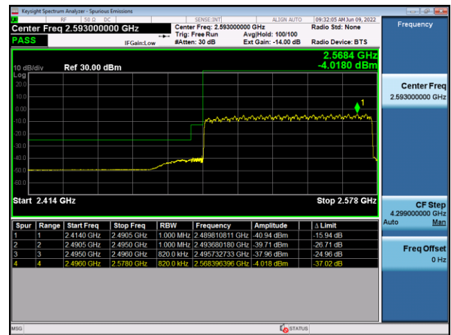
N41(80M)_DFT-s-OFDM_PI/2-BPSK_Edge_ Outer_Full_High_CH
