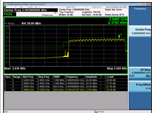
N41(60M)_CP-OFDM_QPSK_Edge_ Outer_Full_Low_CH
