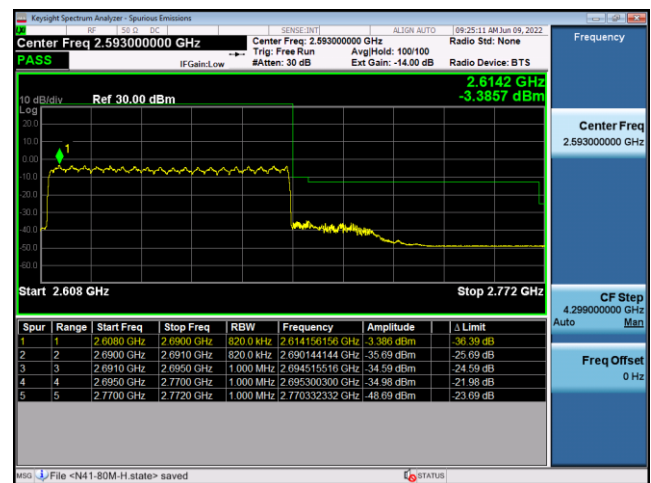
N41(80M)_CP-OFDM_QPSK_Edge_ Outer_Full_High_CH
