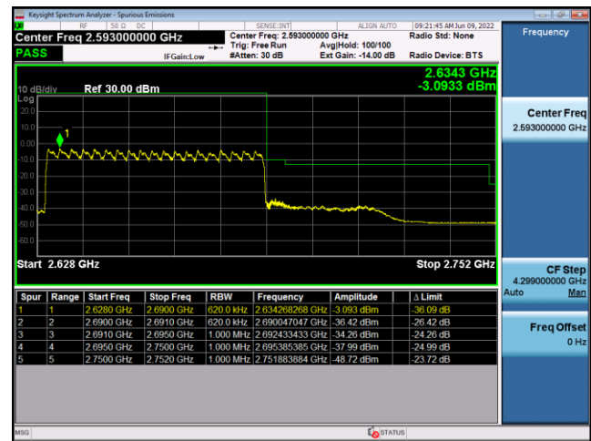
N41(60M)_CP-OFDM_QPSK_Edge_ Outer_Full_High_CH
