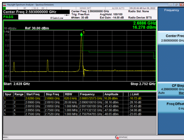
N41(60M)_CP-OFDM_QPSK_Edge_ 1RB_Right_High_CH
