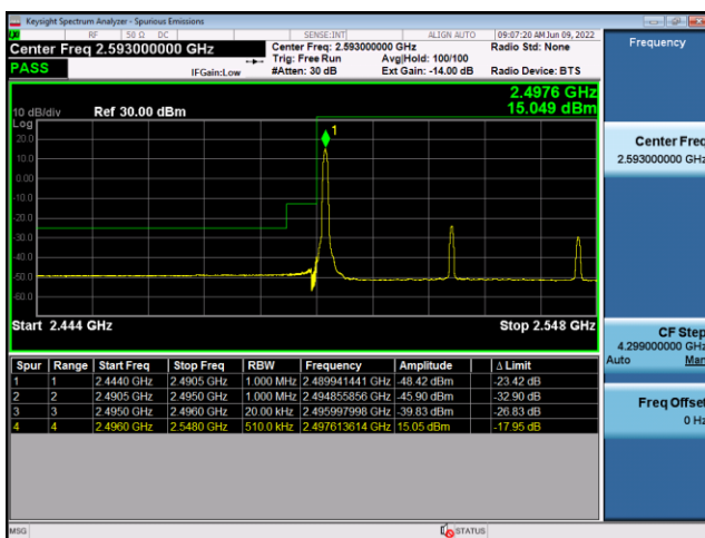
N41(50M)_DFT-s-OFDM_PI/2-BPSK_Edge_ 1RB_Right_High_CH
