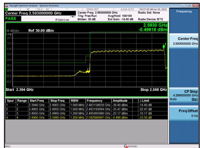
N41(100M)_CP-OFDM_QPSK_Edge_ Outer_Full_Low_CH
