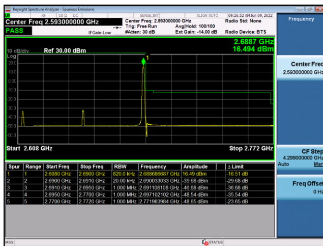
N41(80M)_CP-OFDM_QPSK_Edge_ 1RB_Right_High_CH
