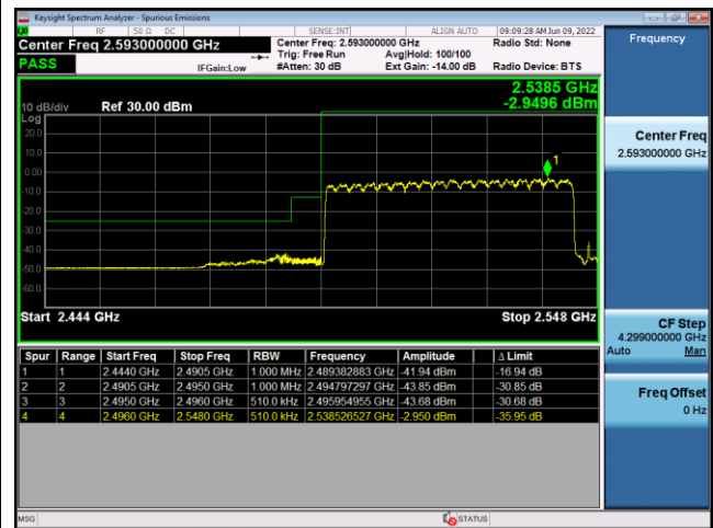
N41(50M)_CP-OFDM_QPSK_Edge_ Outer_Full_Low_CH
