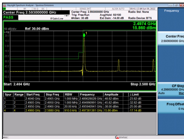
N41(90M)_DFT-s-OFDM_PI/2-BPSK_Edge_ 1RB_Right_High_CH
