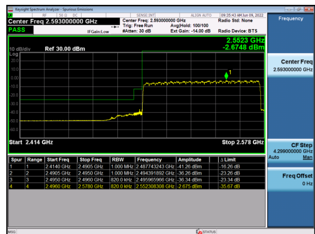
N41(80M)_DFT-s-OFDM_PI/2-BPSK_Edge_ Outer_Full_Low_CH
