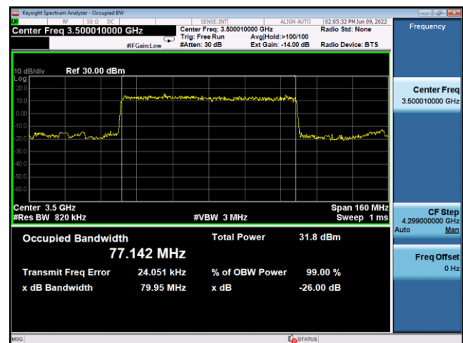
N77(80M)_DFT-s-OFDM_16QAM_ Outer_Full_Mid_CH
