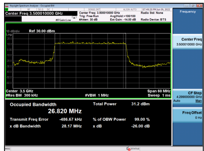
N78(30M)_DFT-s-OFDM_16QAM_ Outer_Full_Mid_CH
