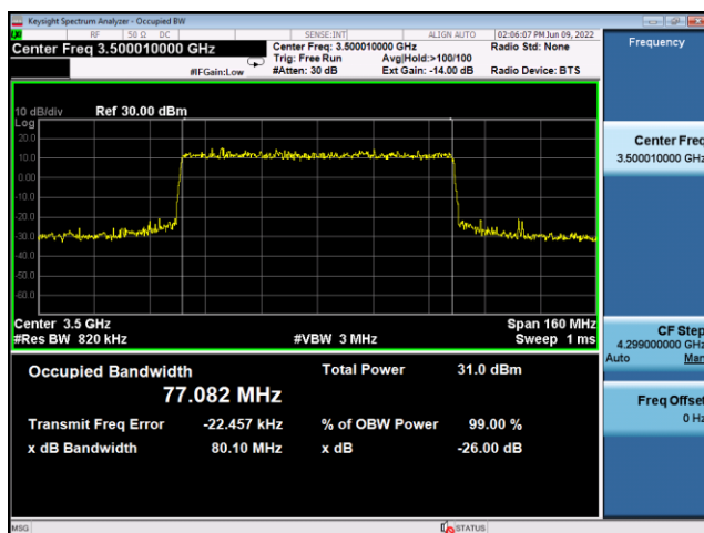
N77(80M)_DFT-s-OFDM_QPSK_ Outer_Full_Mid_CH
