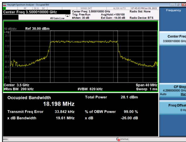
N78(20M)_CP-OFDM_256QAM_ Outer_Full_Mid_CH
