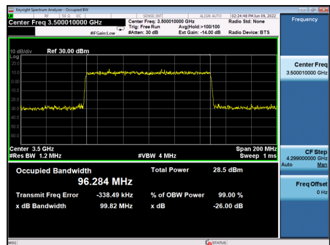
N77(100M)_DFT-s-OFDM_16QAM_ Outer_Full_Mid_CH
