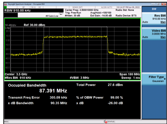
N77(100M)_DFT-s-OFDM_PI_2-BPSK_ Outer_Full_Mid_CH
