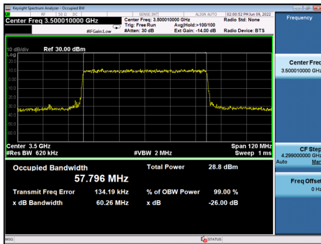
N77(60M)_CP-OFDM_256QAM_ Outer_Full_Mid_CH
