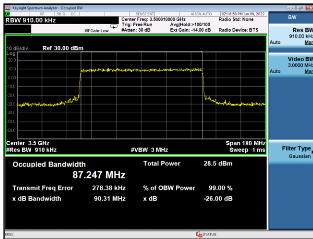
N77(90M)_CP-OFDM_256QAM_ Outer_Full_Mid_CH
