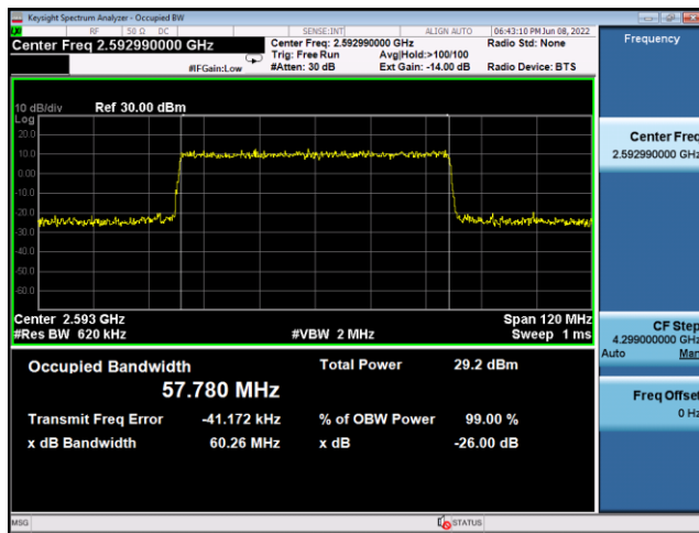
N41(60M)_CP-OFDM_256QAM_ Outer_Full_Mid_CH
