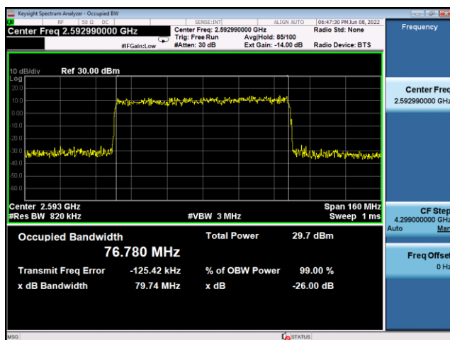
N41(80M)_DFT-s-OFDM_QPSK_ Outer_Full_Mid_CH
