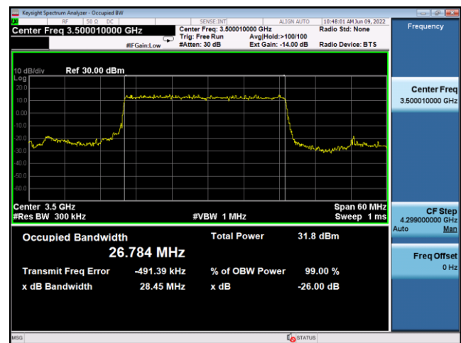
N77(30M)_DFT-s-OFDM_16QAM_ Outer_Full_Mid_CH
