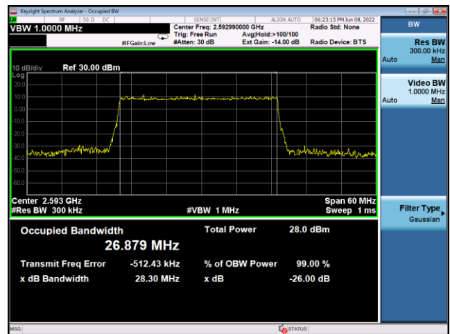
N41(30M)_CP-OFDM_16QAM_ Outer Full Mid_CH
