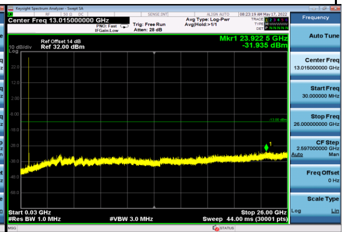
FDD12_LowRange_10MHz_30MHz~26GHz
