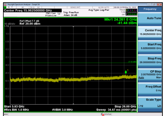
U-NII-3 ,Plot 3,5925MHz~26000MHz-802. 11ax(80MHz),5775MHz,Ant8
