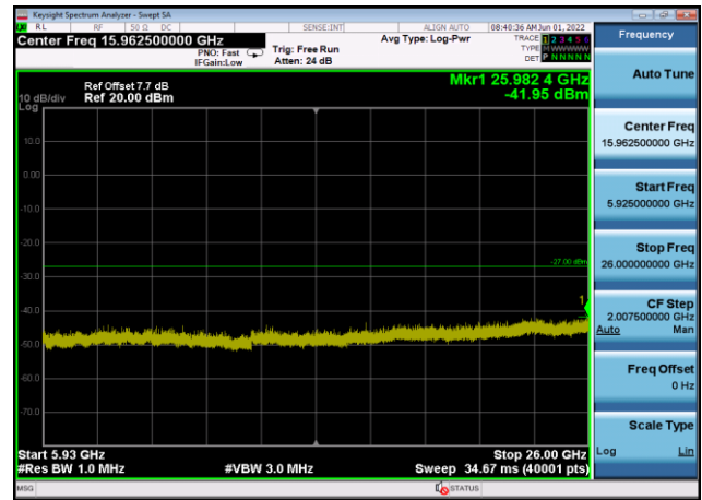
U-NII-3 ,Plot 3,5925MHz~26000MHz-802. 11a(20MHz),5785MHz,Ant8
