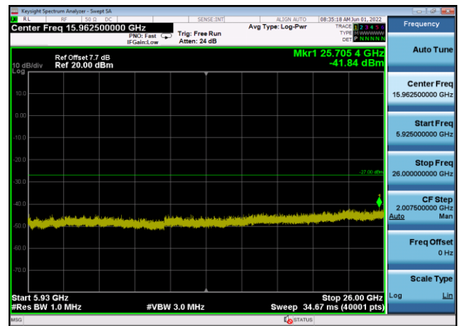
U-NII-3 ,Plot 3,5925MHz~26000MHz-802. 11a(20MHz),5825MHz,Ant8
