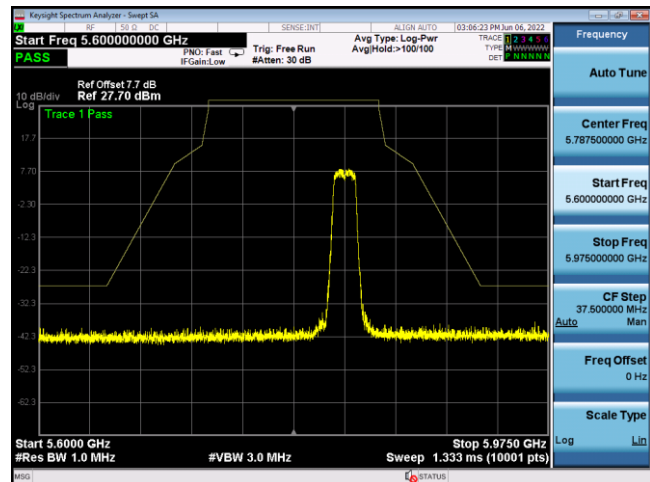
U-NII-3 ,Plot 1,Band Edge-802.11a(20 Hz),5825MHz,Ant8
