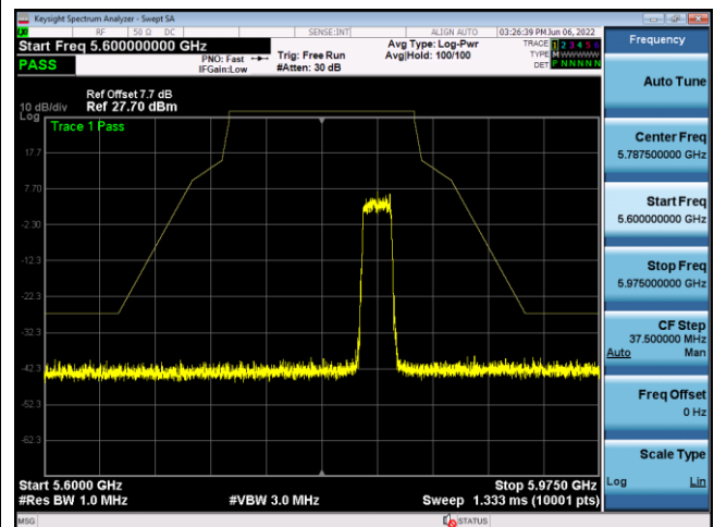
U-NII-3 ,Plot 1,Band Edge-802.11ax(20 MHz),5825MHz,Ant8
