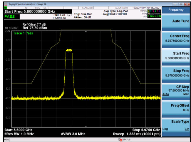
U-NII-3 ,Plot 1,Band Edge-802.11a(20 Hz),5785MHz,Ant8
