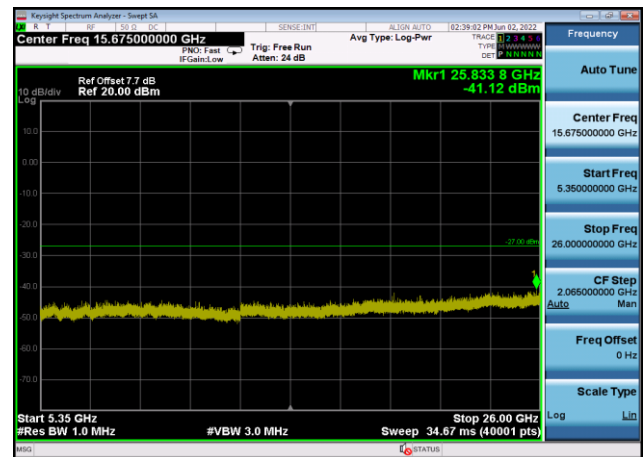
U-NII-2a ,Plot 3,5350MHz~26000MHz-802 .11ax(160MHz),5250MHz,Ant8
