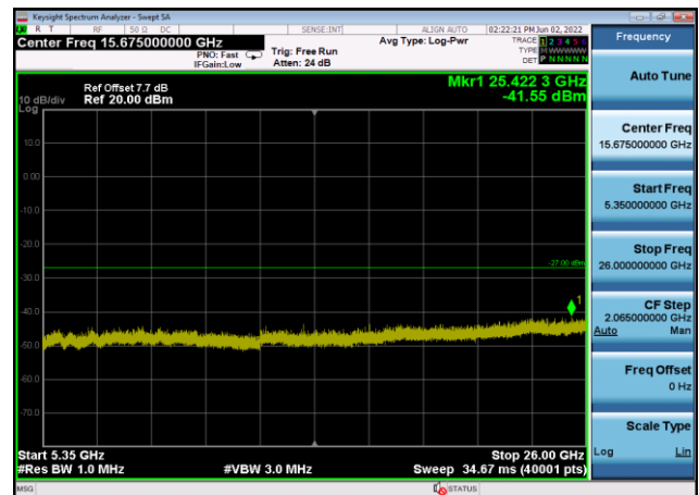
U-NII-2a ,Plot 3,5350MHz~26000MHz-802 .11ax(80MHz),5290MHz,Ant8
