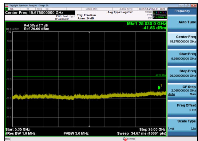
U-NII-2a ,Plot 3,5350MHz~26000MHz-802 .11a(20MHz),5300MHz,Ant8
