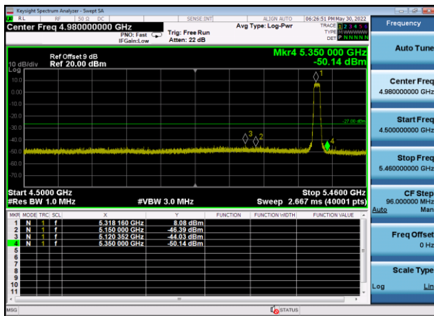
U-NII-2a ,Plot 1,Band Edge-802.11a(20 MHz),5320MHz,Ant9
