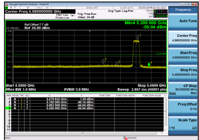
U-NII-2a ,Plot 1,Band Edge-802.11n(40 MHz),5310MHz,Ant8
