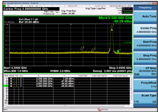
U-NII-2a ,Plot 1,Band Edge-802.11a(20 MHz),5320MHz,Ant8
