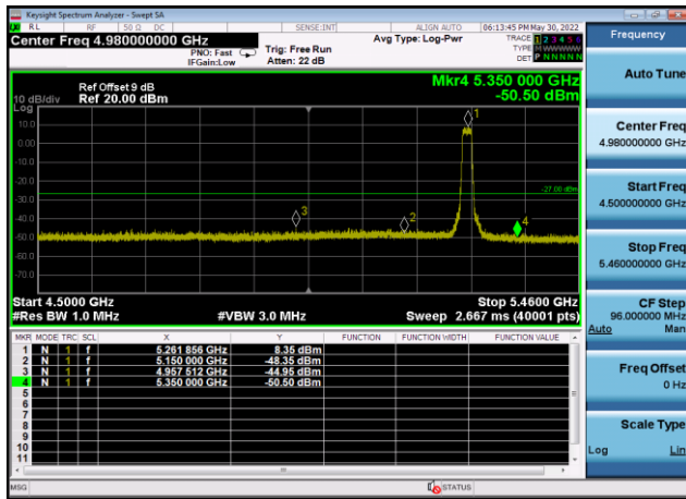
U-NII-2a ,Plot 1,Band Edge-802.11a(20 MHz),5300MHz,Ant9
