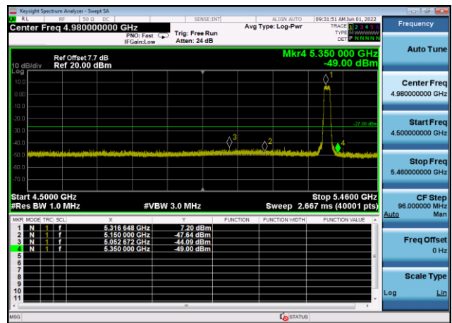
U-NII-2a ,Plot 1,Band Edge-802.11a(20 MHz),5320MHz,Ant8
