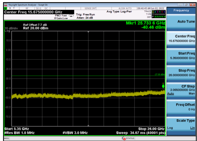
U-NII-1 ,Plot 3,5350MHz~26000MHz-802. 11ax(20MHz),5240MHz,Ant8
