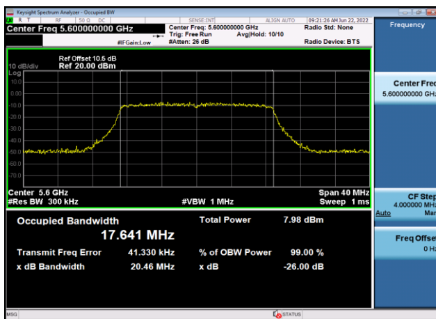
U-NII-2c 99% Bandwidth-802.11ac(20MHz),5600MHz,Ant9
