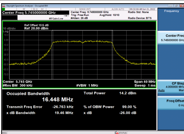
U-NII-3 99% Bandwidth-802.11a(20MHz) ,5745MHz,Ant9
