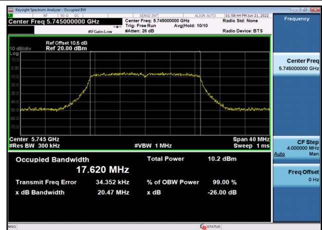
U-NII-3 99% Bandwidth-802.11ac(20MHz) ,5745MHz,Ant8
