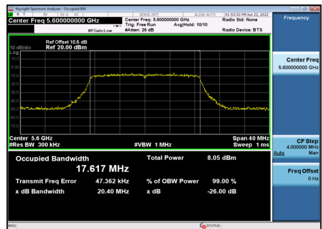
U-NII-2c 99% Bandwidth-802.11ac(20MHz),5600MHz,Ant8
