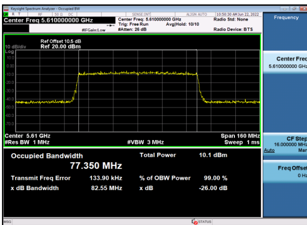
U-NII-2c 99% Bandwidth-802.11ax(80MHz ) ,5610MHz,Ant9
