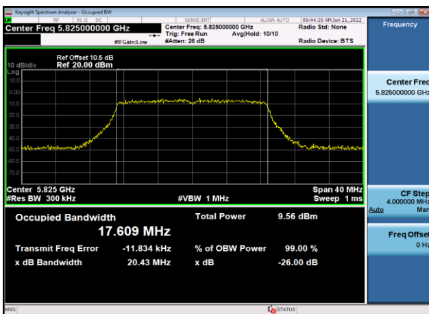
U-NII-3 99% Bandwidth-802.11n(20MHz) ,5825MHz,Ant9
