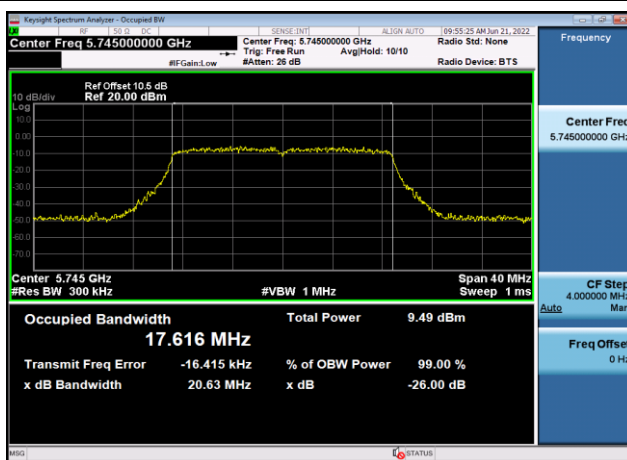
U-NII-3 99% Bandwidth-802.11ac(20MHz) ,5745MHz,Ant9
