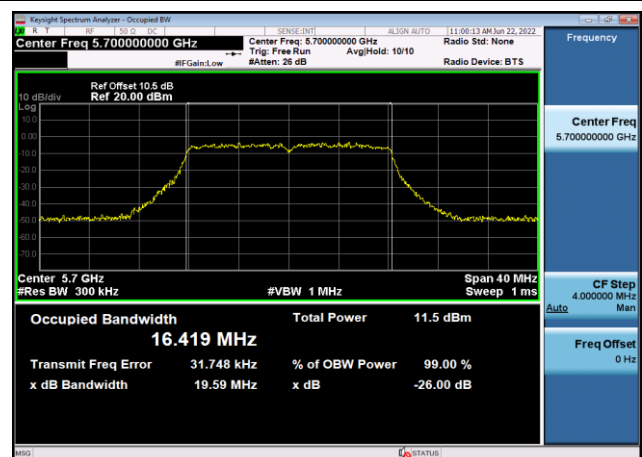
U-NII-2c 99% Bandwidth-802.11a(20MHz) ,5700MHz,Ant8
