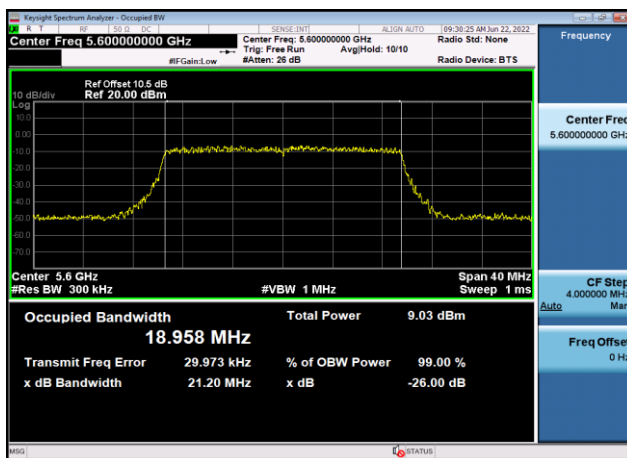
U-NII-2c 99% Bandwidth-802.11ax(20MHz),5600MHz,Ant9
