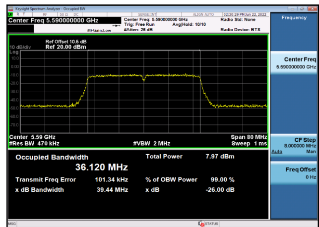
U-NII-2c 99% Bandwidth-802.11ac(40MHz ,5590MHz,Ant8
