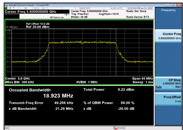
U-NII-2c 99% Bandwidth-802.11ax(20MHz),5600MHz,Ant8
