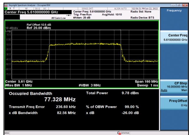
U-NII-2c 99% Bandwidth-802.11ax(80MHz ) ,5610MHz,Ant8
