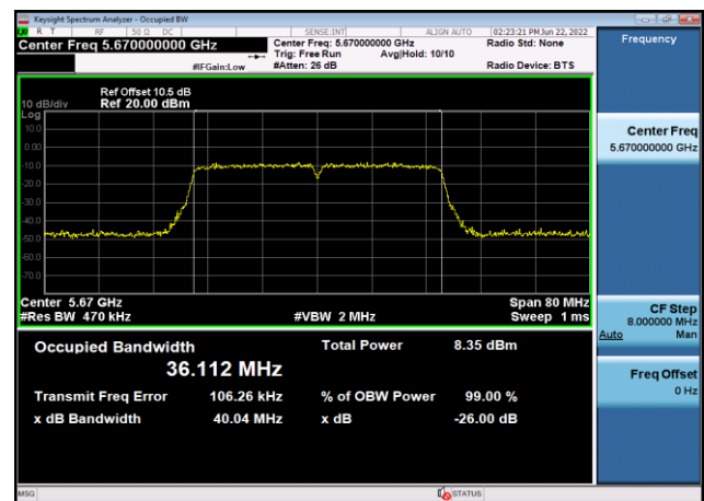
U-NII-2c 99% Bandwidth-802.11n(40MHz) ,5670MHz,Ant8
