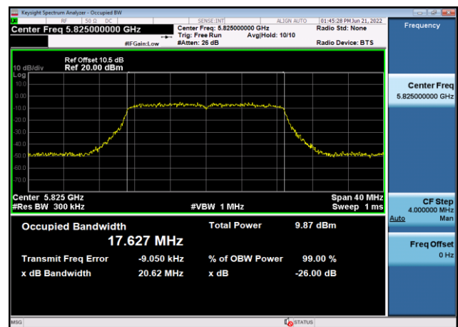
U-NII-3 99% Bandwidth-802.11n(20MHz) ,5825MHz,Ant8
