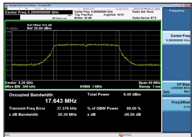
U-NII-2a 99% Bandwidth-802.11ac(20MHz) ,5260MHz,Ant8
