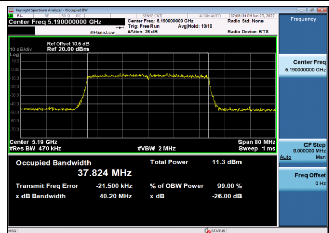
U-NII-1 99% Bandwidth-802.11ax(40MHz) ,5190MHz,Ant8
