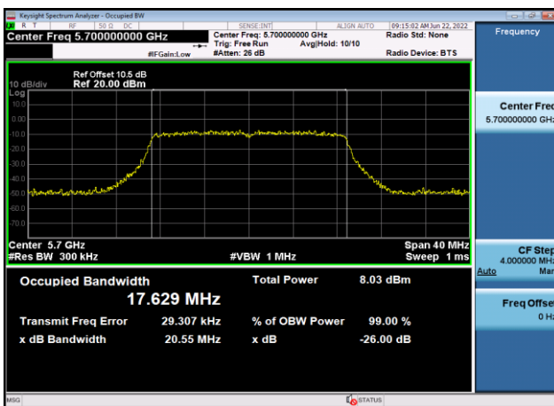
U-NII-2c 99% Bandwidth-802.11n(20MHz) ,5700MHz,Ant9
