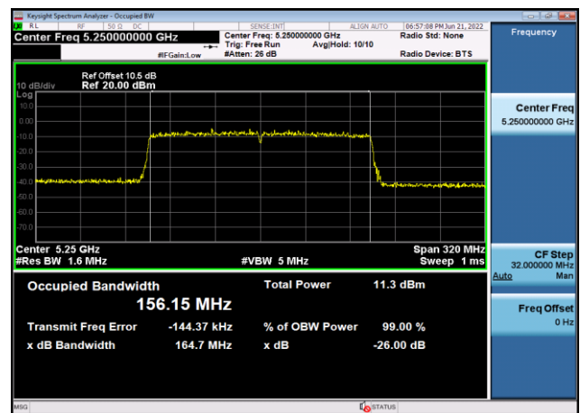
U-NII-2a 99% Bandwidth-802.11ax(160MH z),5250MHz,Ant8
