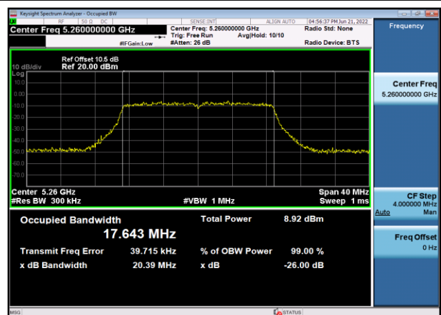
U-NII-2a 99% Bandwidth-802.11n(20MHz) ,5260MHz,Ant8
