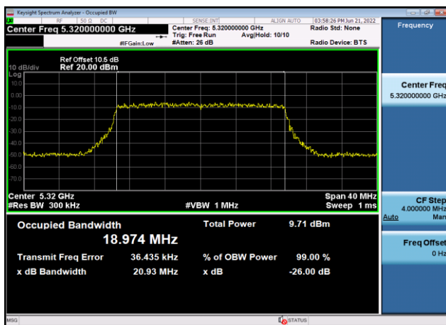
U-NII-2a 99% Bandwidth-802.11ax(20MHz )5320MHz,Ant9
