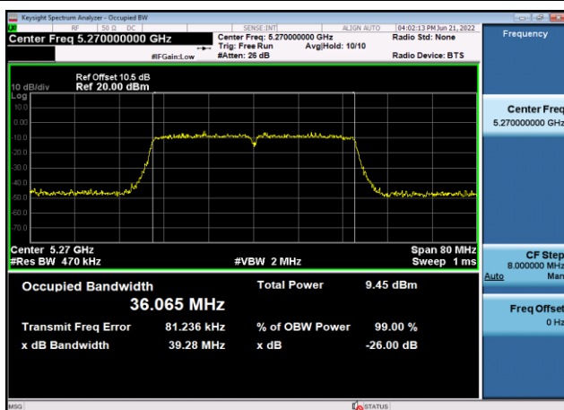
U-NII-2a 99% Bandwidth-802.11n(40MHz) ,5270MHz,Ant9
