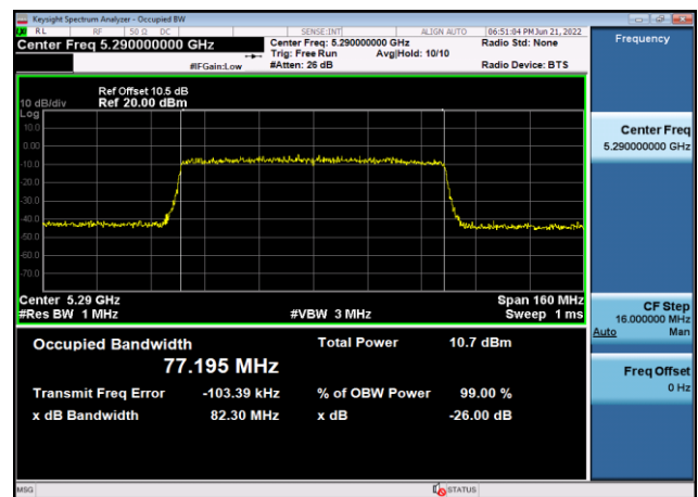
U-NII-2a 99% Bandwidth-802.11ax(80MHz )5290MHz,Ant8
