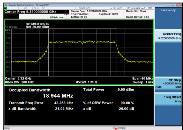
U-NII-2a 99% Bandwidth-802.11ax(20MHz )5320MHz,Ant8
