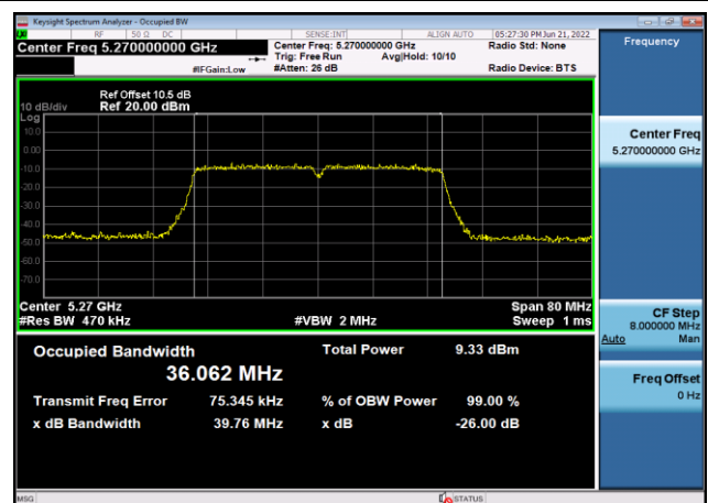
U-NII-2a 99% Bandwidth-802.11n(40MHz) ,5270MHz,Ant8
