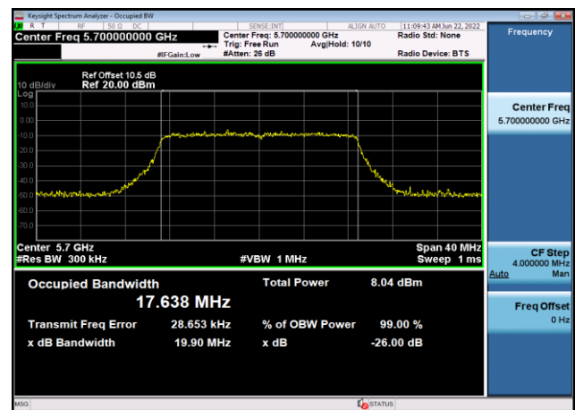
U-NII-2c 99% Bandwidth-802.11n(20MHz) ,5700MHz,Ant8
