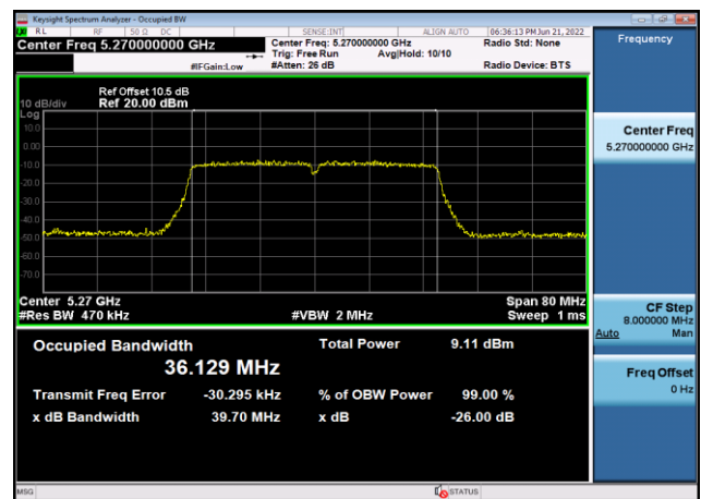
U-NII-2a 99% Bandwidth-802.11ac(40MHz )5270MHz,Ant8
