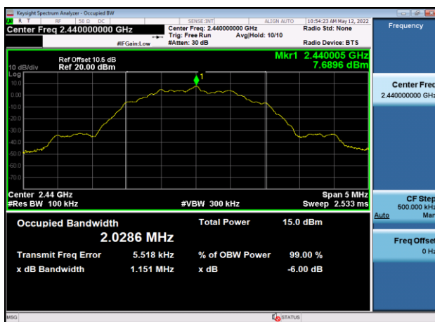
6dB Bandwidth: 2440MHz – 2MHz bandwidth
