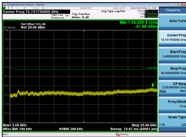
,Plot 4,2483.5MHz~25000MHz-802.11ax(H T40),2452MHz,Ant9
