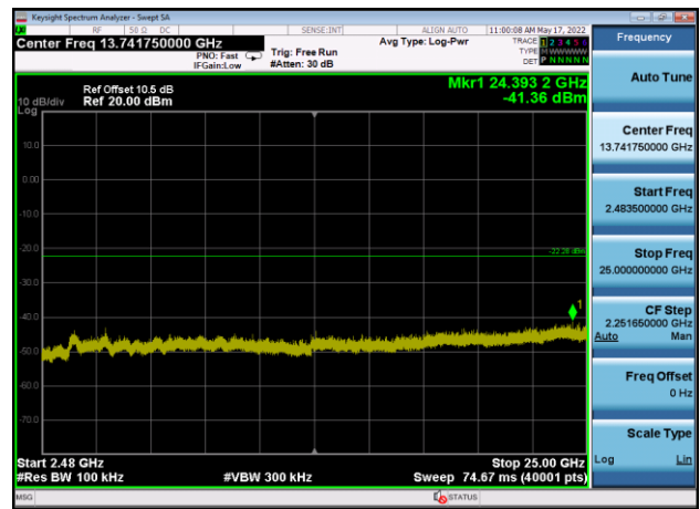
,Plot 4,2483.5MHz~25000MHz-802.11ax(H T40),2437MHz,Ant7
