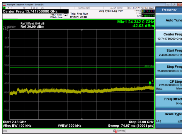
,Plot 4,2483.5MHz~25000MHz-802.11ax(H T40),2437MHz,Ant9
