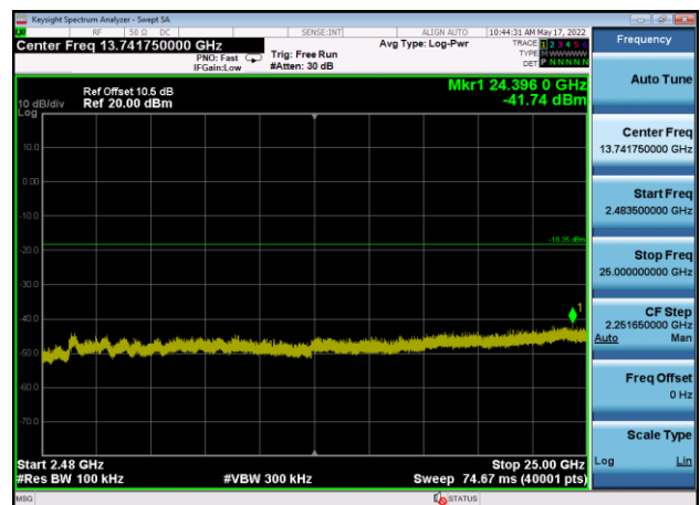
,Plot 4,2483.5MHz~25000MHz-802.11ax(H T20),2462MHz,Ant7
