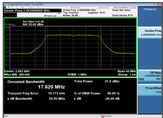
99% Bandwidth-802.11n(HT20),2462MHz ,Ant7
