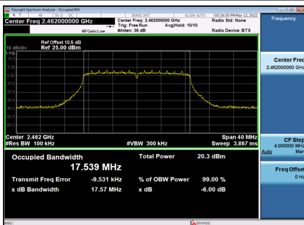
6dB Bandwidth-802.11n(HT20),2462MHz
