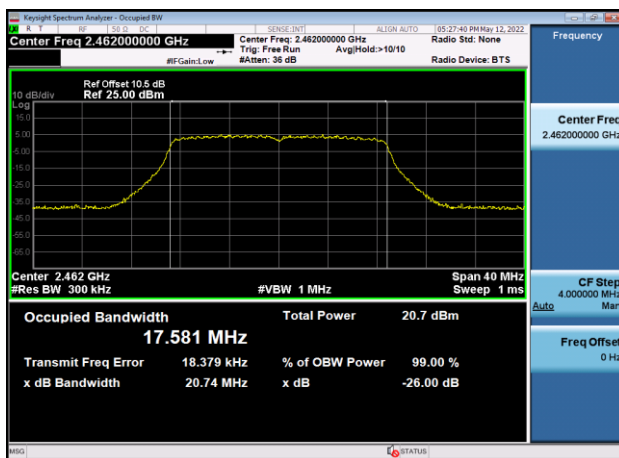
99% Bandwidth-802.11n(HT20),2462MHz ,Ant9
