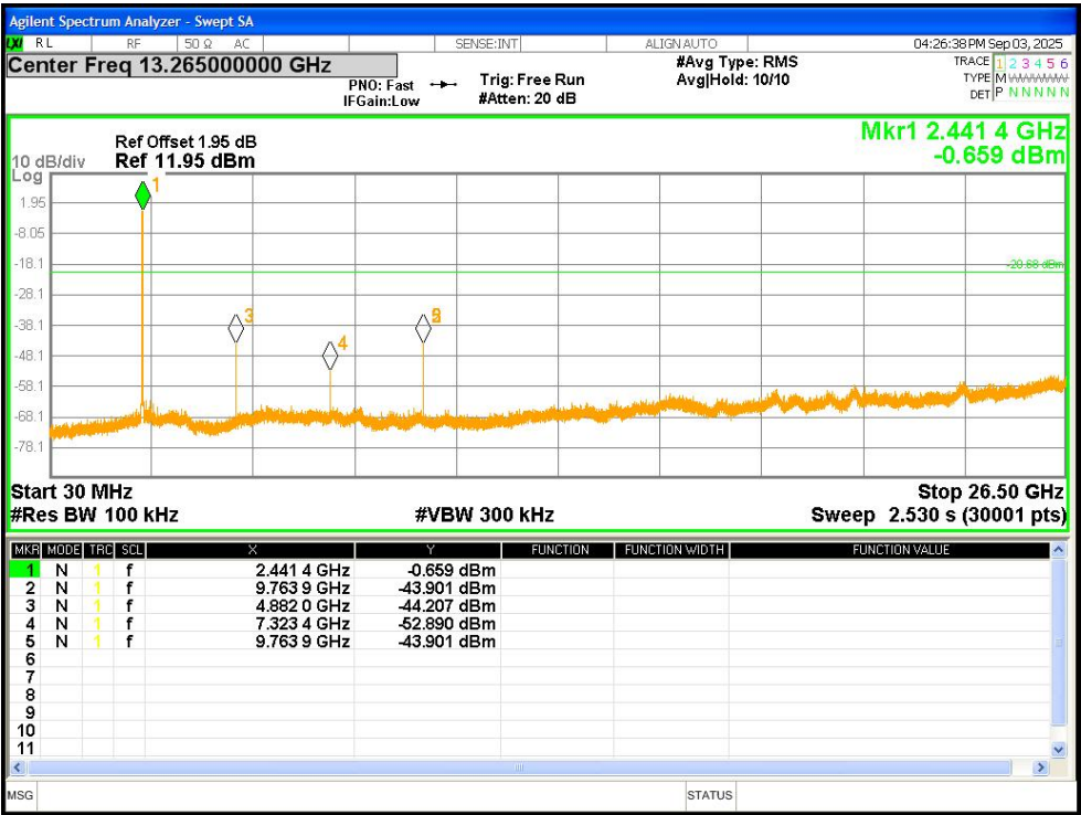
Tx. Spurious NVNT 1-DH5 2441MHz Ant1
