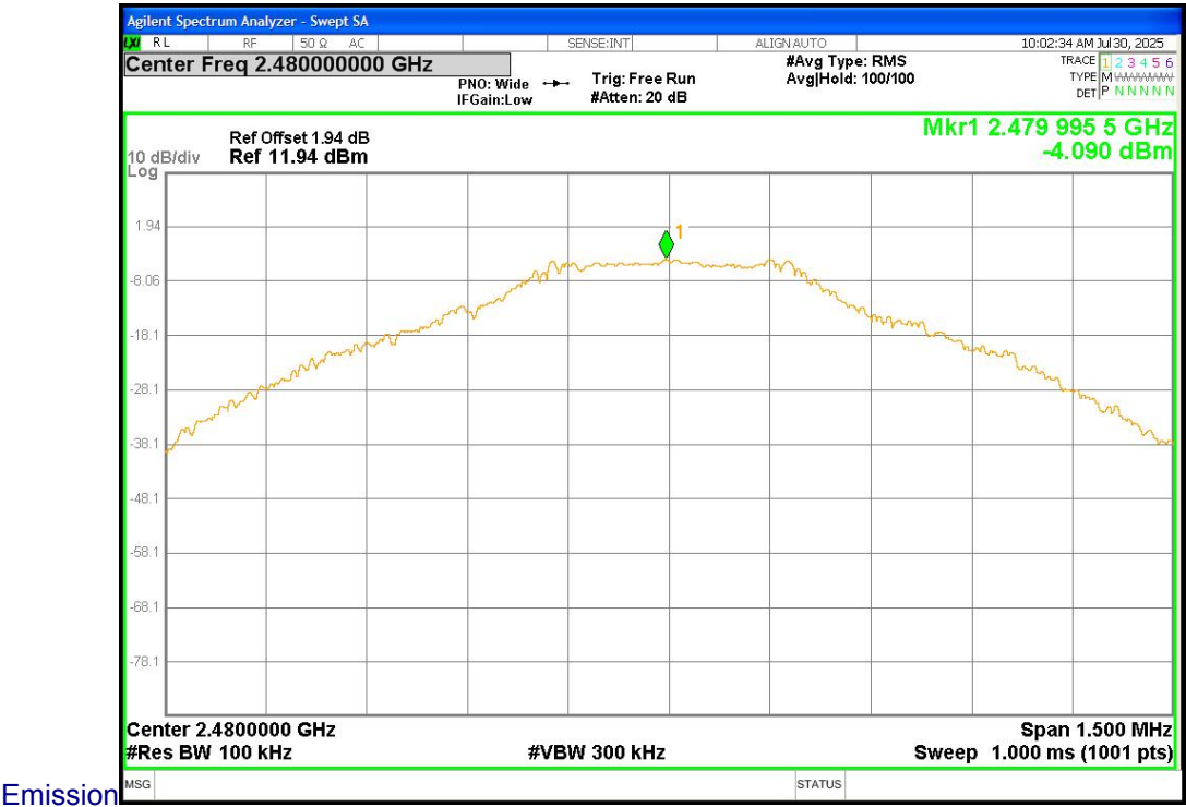
Emission Tx. Spurious NVNT 1-DH5 2480MHz Ant1 Ref
