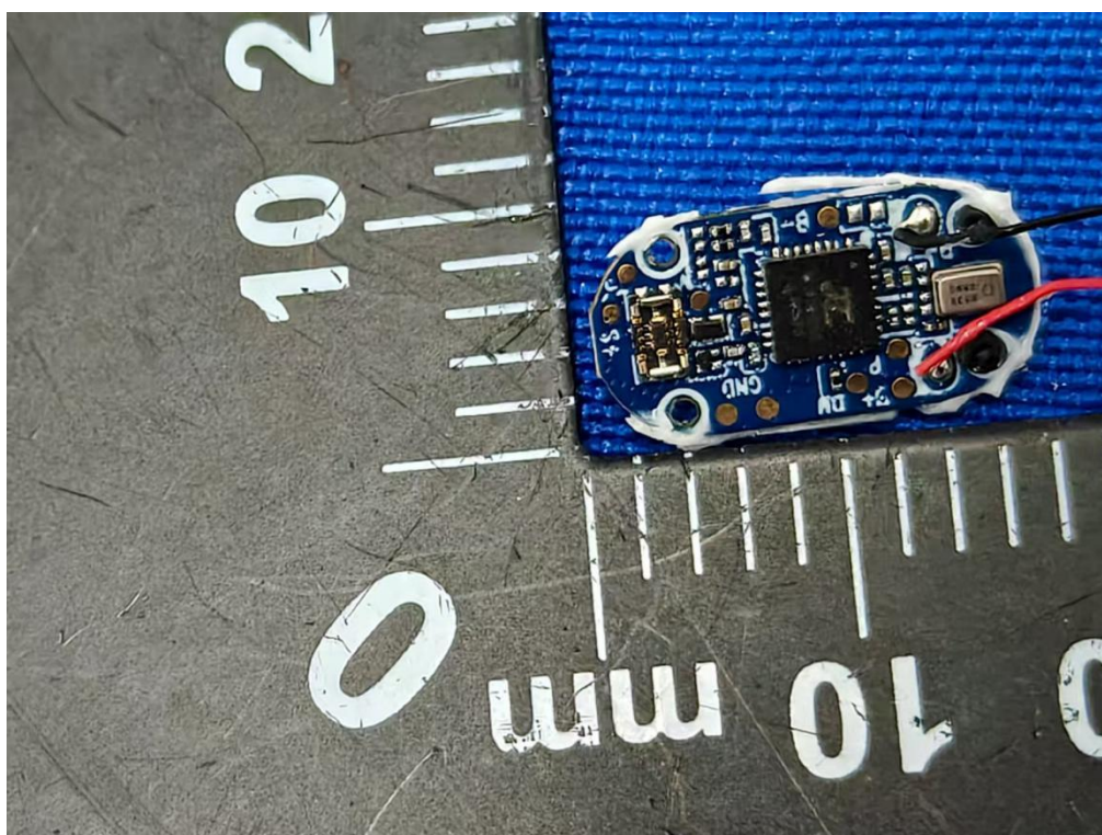
PCB view of unit (Model: Rooftop Shark AI-10; HVIN: Rooftop Shark AI-10)
