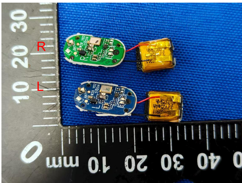
Internal view of unit (Model: Rooftop Shark AI-10; HVIN: Rooftop Shark AI-10)
