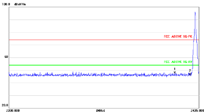
2432MHz Vertical
