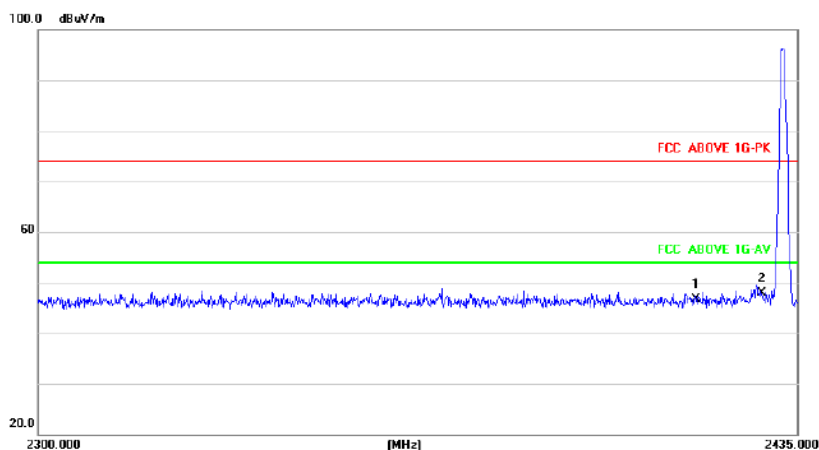
2432MHz Horizontal
