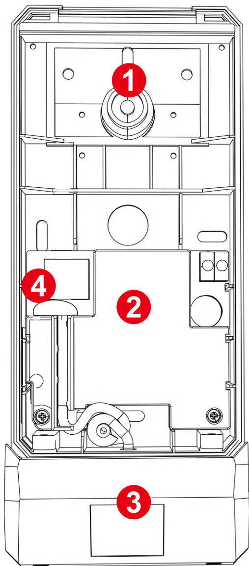
CT9-T/H-QP Installation Plate
