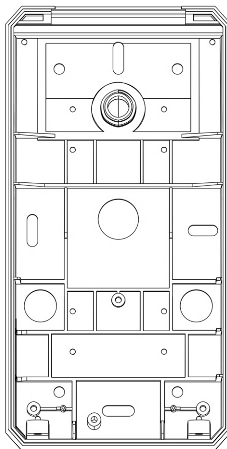
CT9-M(E)-T Installation Plate
