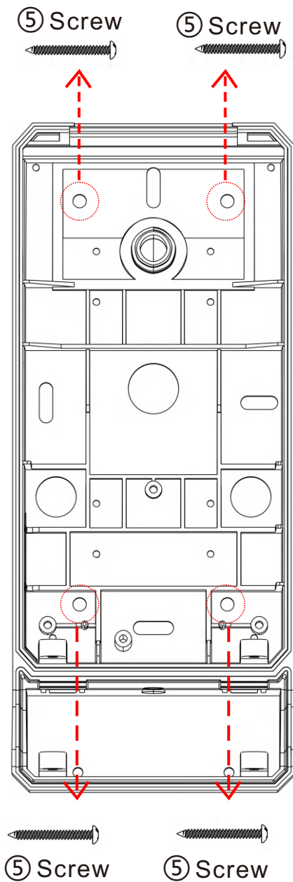
TYPE 1 of Installation Hole
