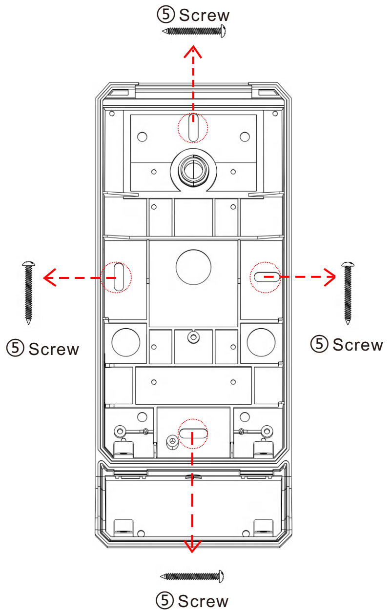
TYPE 2 of Installation Hole
