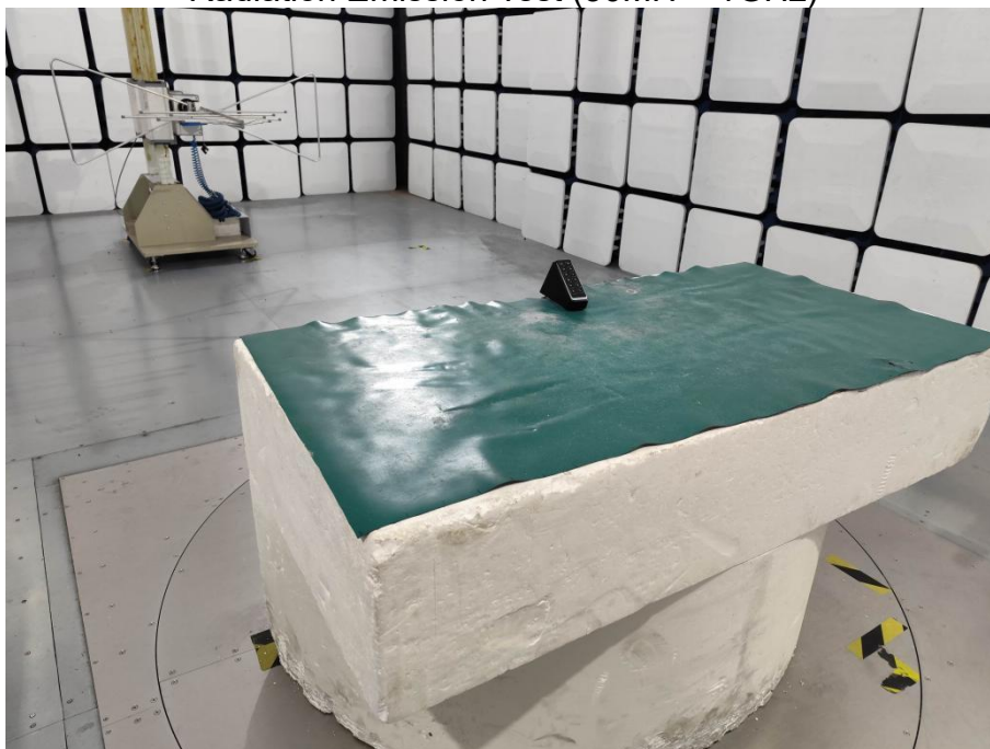
Radiation Emission Test (30MH ~ 1GHz)
