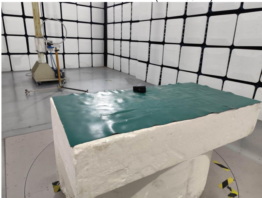
Radiation Emission Test (below 30MH)
