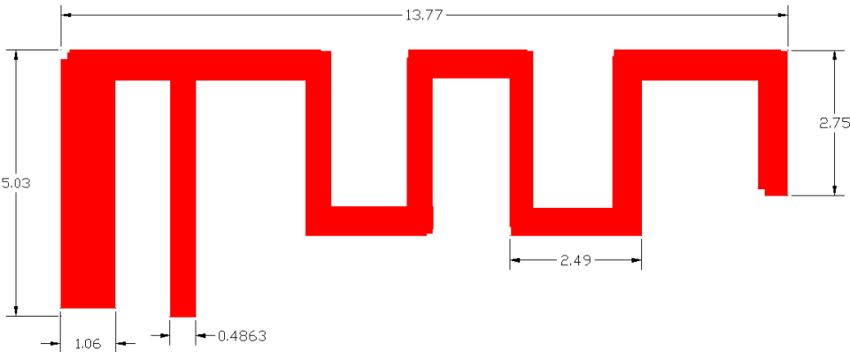
Antenna Photo & Lenght( mm)
