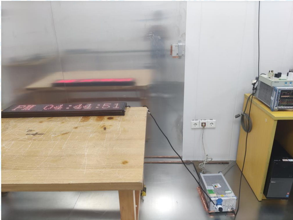
Photo of Setup for Conducted Emission
