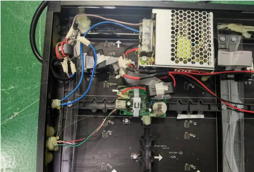
Photo 5 Internal of EUT
