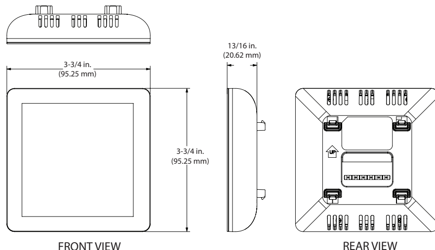
Figure 2. Thermostat Dimensions
