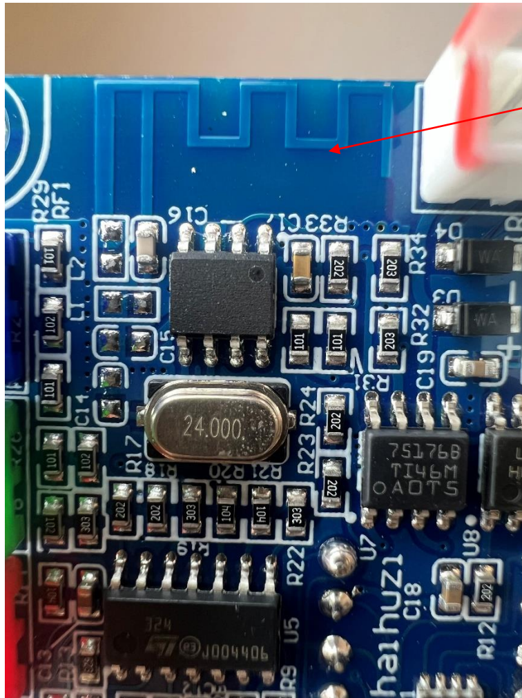
BT Antenna
