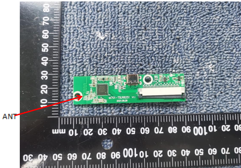
Internal Photo FCC ID: 2A6ES-DK61
