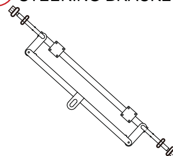
STEERING BRACKET
