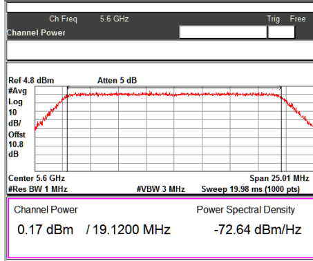
Channel frequency:5600MHz@Chain2
