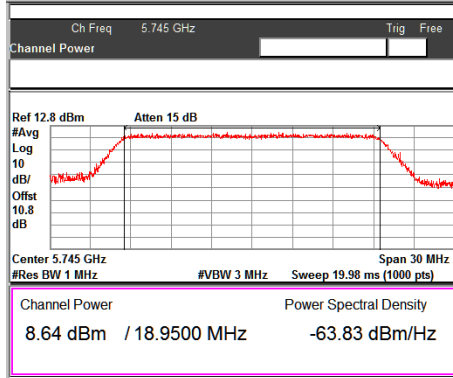
Channel frequency:5745MHz@Chain2
