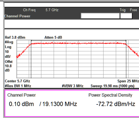
Channel frequency:5700MHz@Chain2
