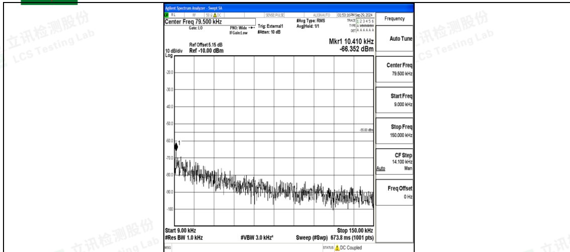
Band41_10MHz_16QAM_40620_1RB#0_0.009~0.15_0.009~0.15
