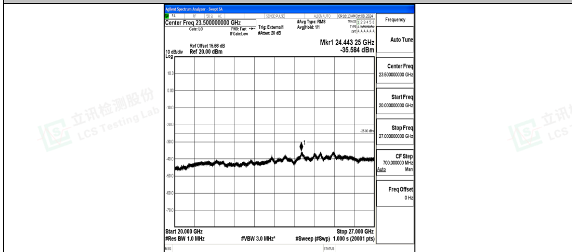
Band38_5MHz_QPSK_38000_1RB#0_20000~27000_20000~27000
