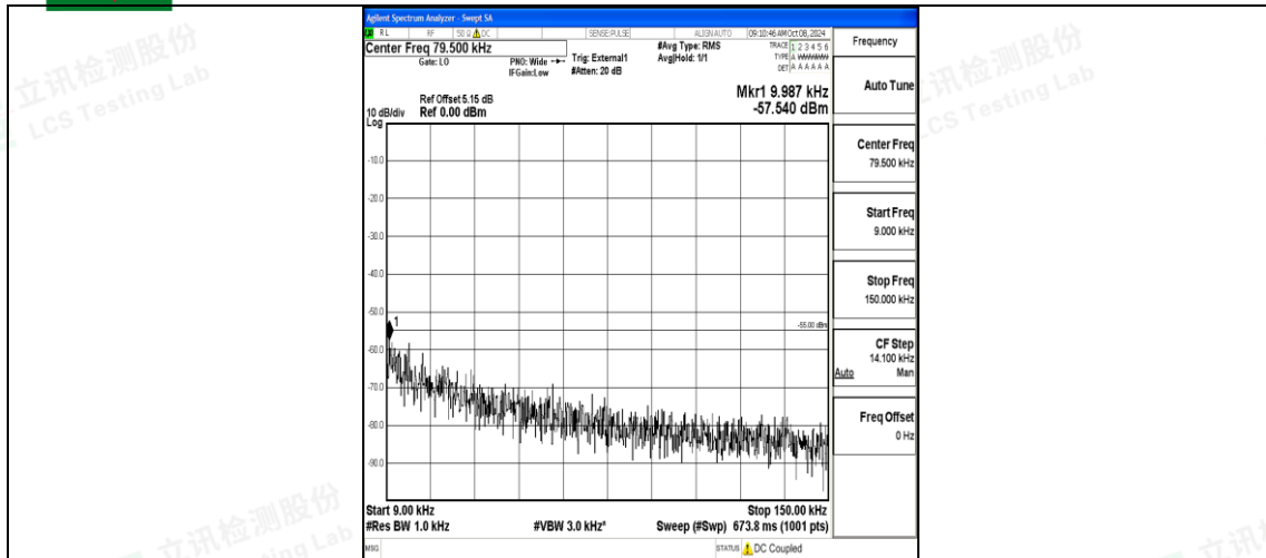
Band38_5MHz_QPSK_37775_1RB#0_0.009~0.15_0.009~0.15
