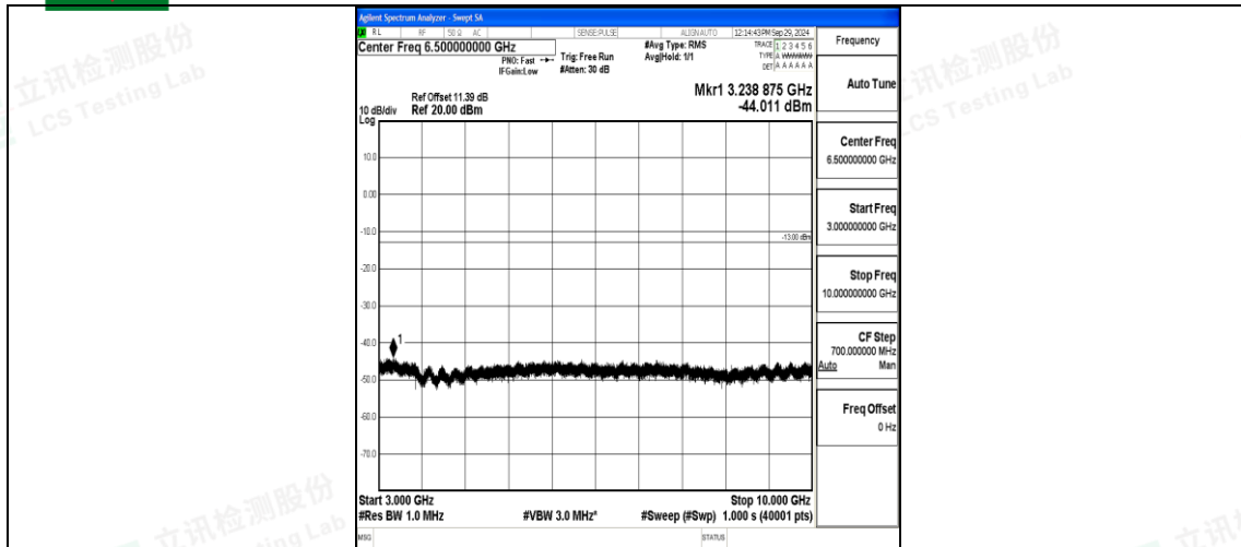
Band12_10MHz_QPSK_23130_1RB#0_3000~10000_3000~10000
