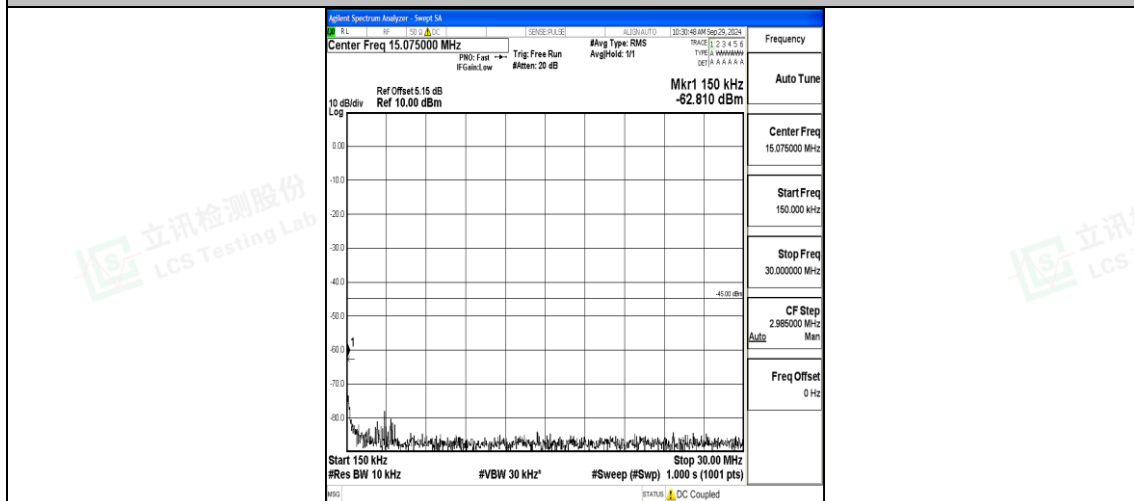
Band7_15MHz_16QAM_21375_1RB#0_0.15~30_0.15~30
