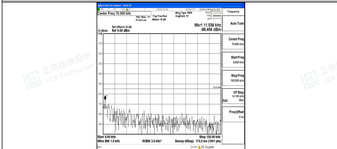
Band7_20MHz_QPSK_21350_1RB#0_0.009~0.15_0.009~0.15
