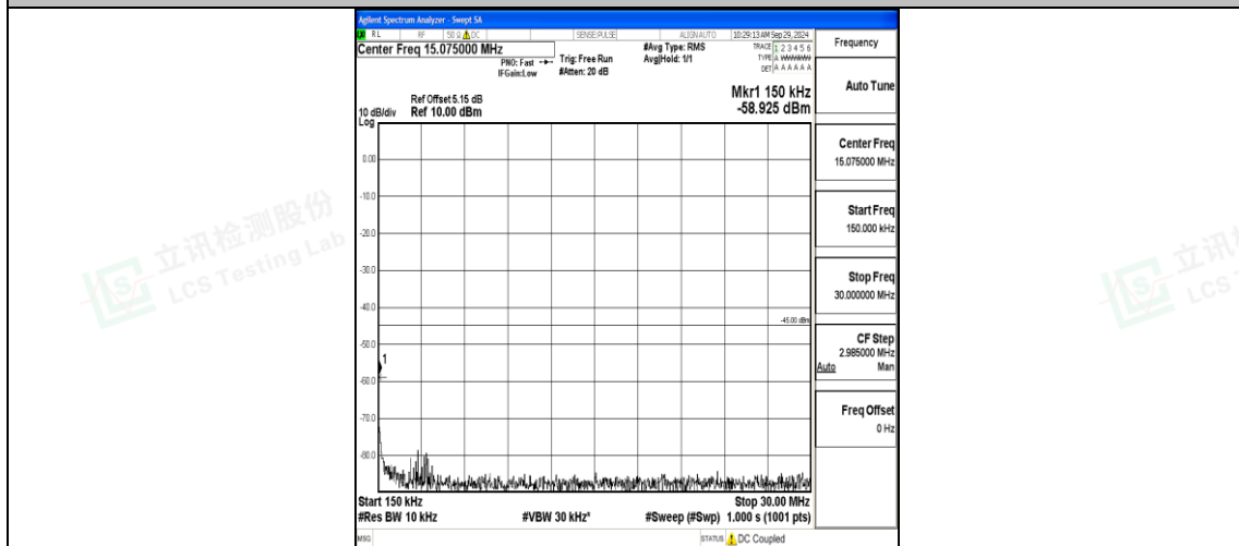
Band7_15MHz_QPSK_21100_1RB#0_0.15~30_0.15~30
