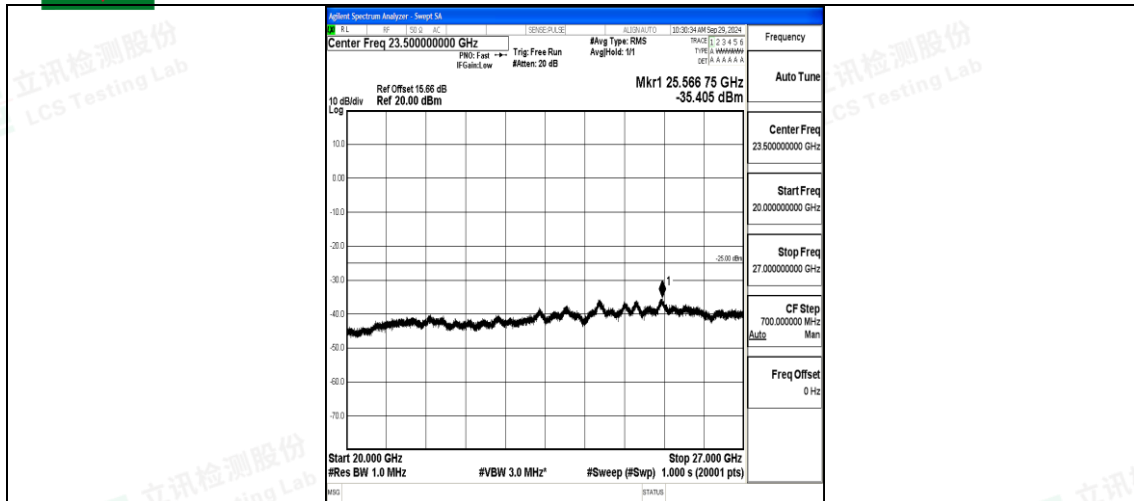
Band7_15MHz_QPSK_21375_1RB#0_20000~27000_20000~27000
