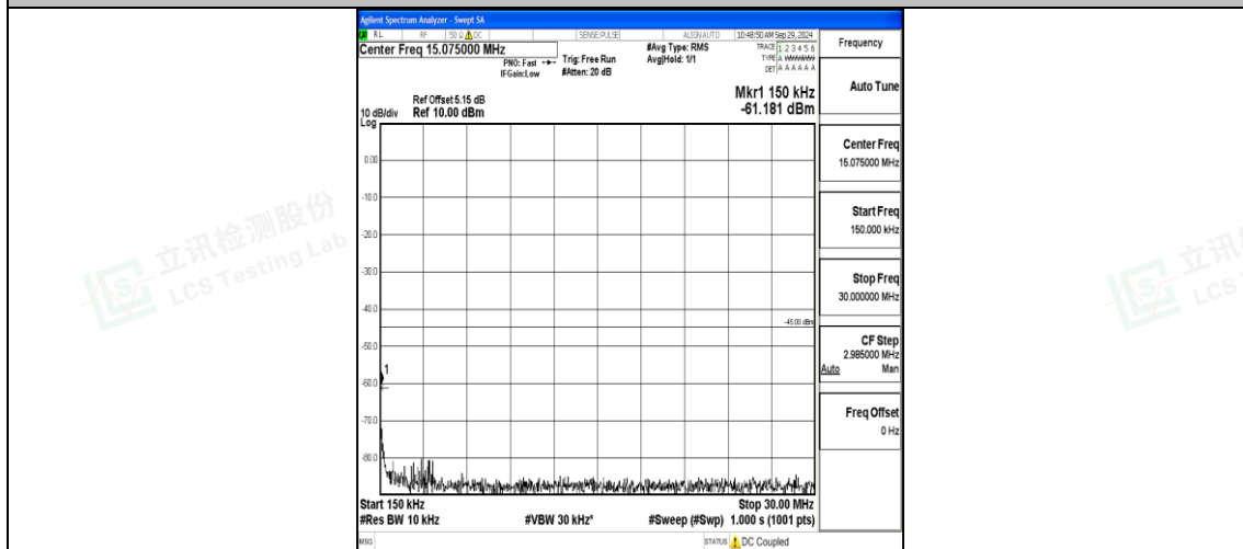
Band7_20MHz_16QAM_21350_1RB#0_0.15~30_0.15~30
