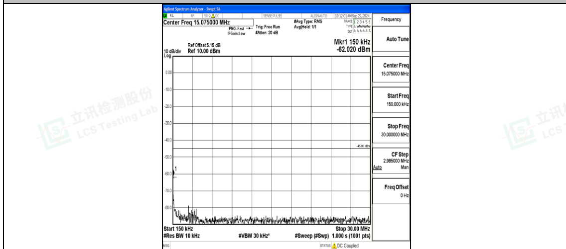
Band7_10MHz_QPSK_21100_1RB#0_0.15~30_0.15~30
