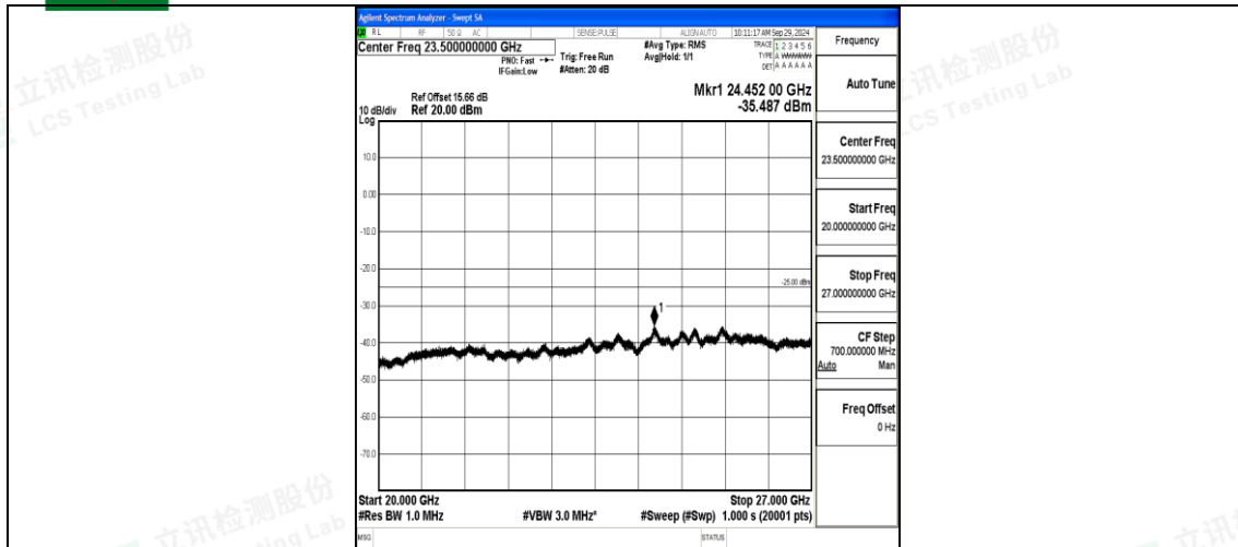
Band7_10MHz_QPSK_20800_1RB#0_20000~27000_20000~27000
