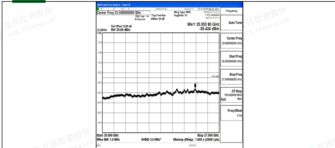
Band7_10MHz_16QAM_20800_1RB#0_20000~27000_20000~27000
