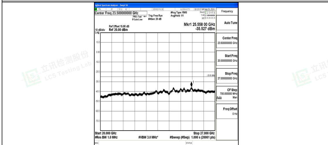
Band7_10MHz_QPSK_21400_1RB#0_20000~27000_20000~27000
