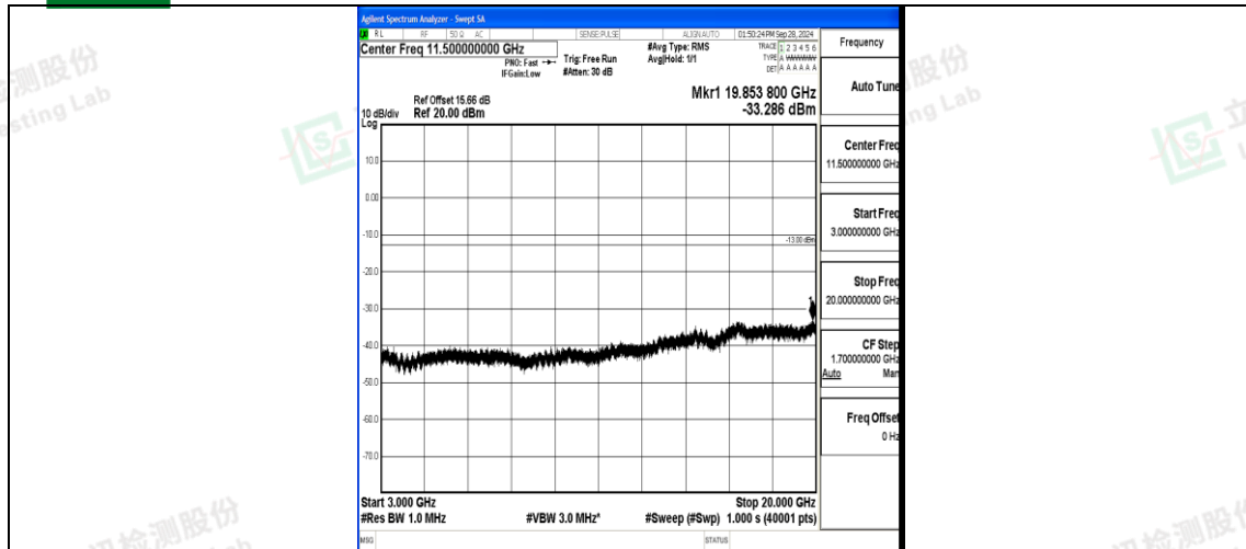
Band4_1.4MHz_16QAM_20393_1RB#0_3000~20000_3000~20000
