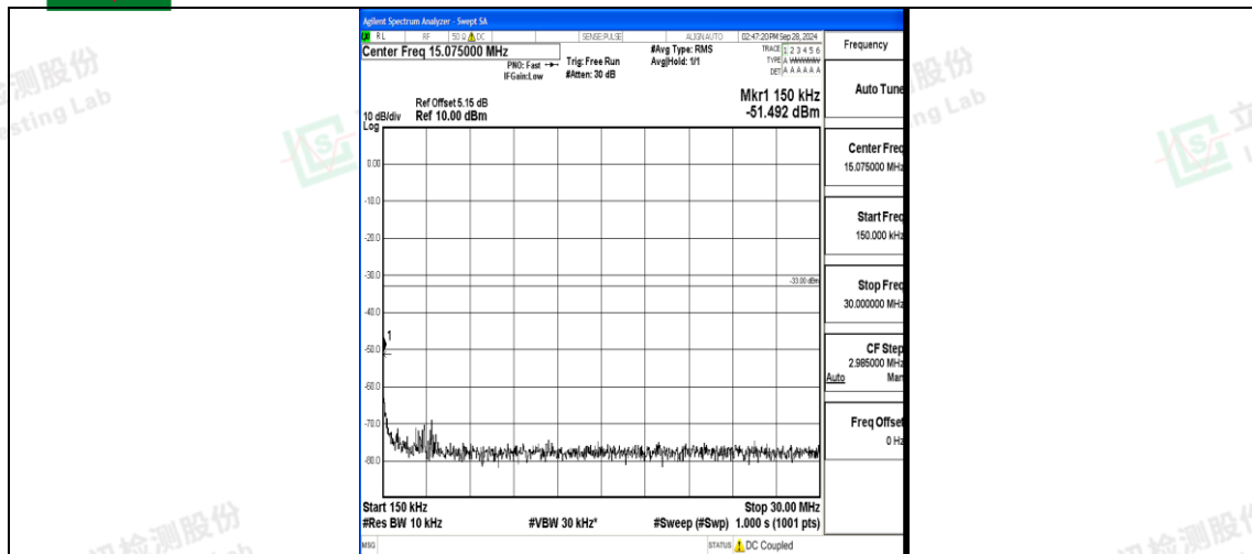
Band4_10MHz_16QAM_20175_1RB#0_0.15~30_0.15~30
