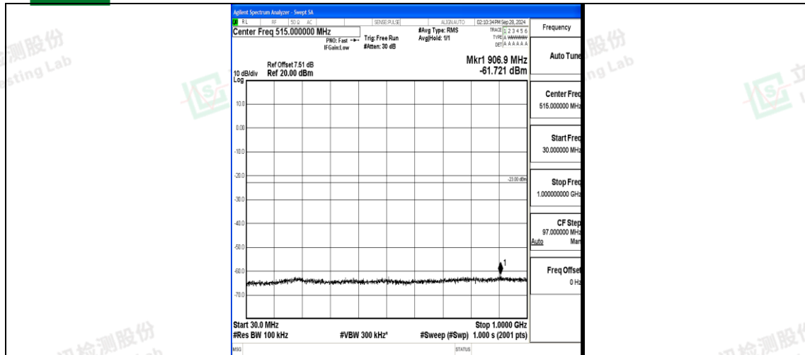
Band4_3MHz_QPSK_19965_1RB#0_30~1000_30~1000
