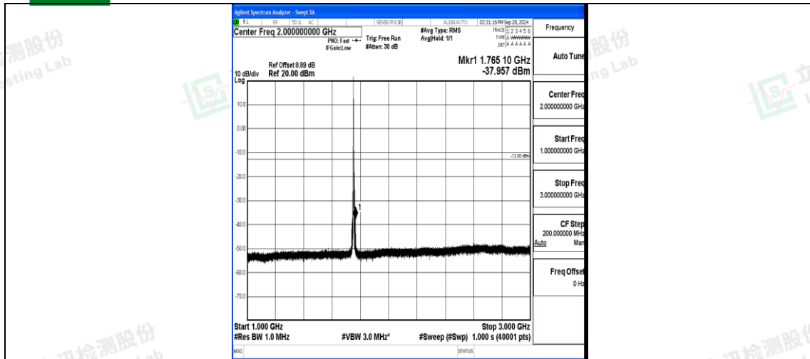
Band4_5MHz_16QAM_20375_1RB#0_1000~3000_1000~3000
