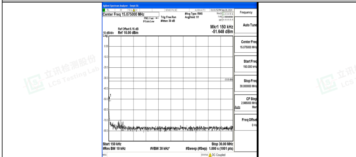
Band2_10MHz_16QAM_19150_1RB#0_0.15~30_0.15~30
