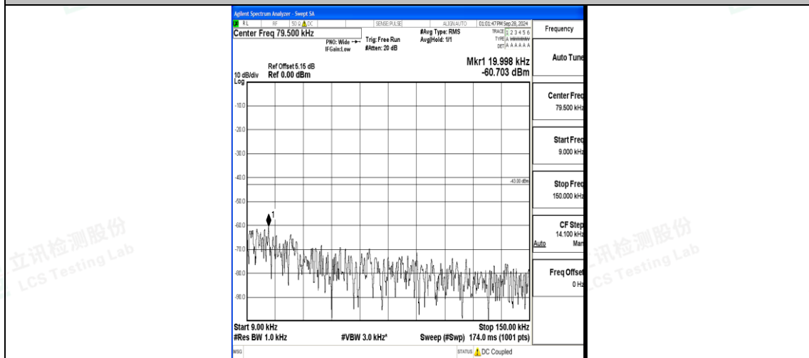
Band2_10MHz_16QAM_19150_1RB#0_0.009~0.15_0.009~0.15
