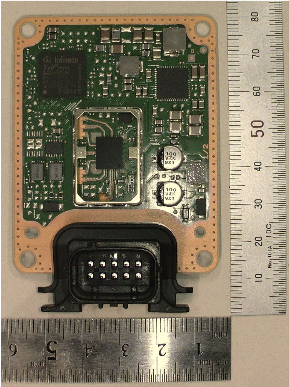
Component side A
