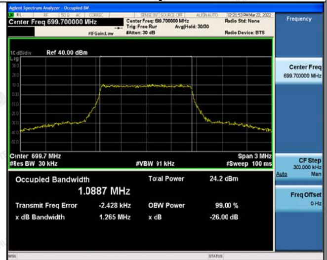
16QAM
