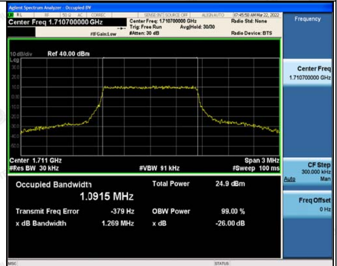
16QAM
