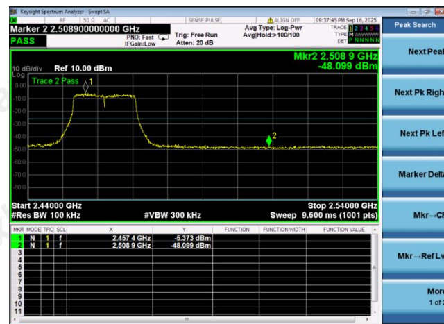
Right bandedge
