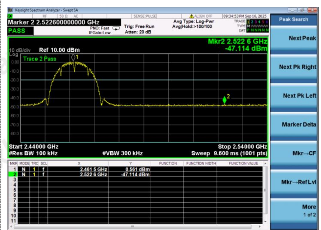
Right bandedge
