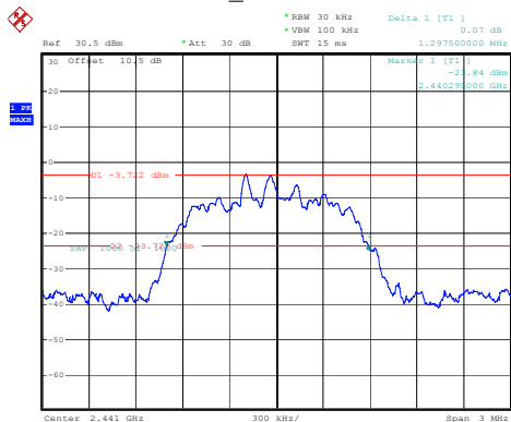
2DH1_Middle 1.298MHz
