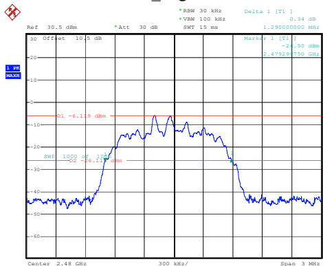
2DH1_High 1.290MHz
