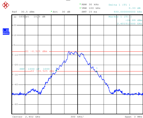
DH1_Low 0.930MHz
