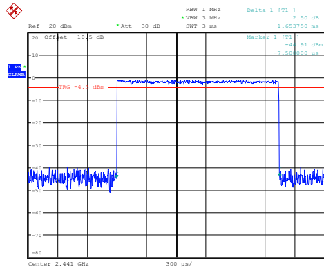
2DH3_Hopping 1.654ms
