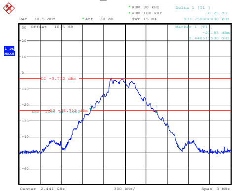
DH1_Middle 0.934MHz
