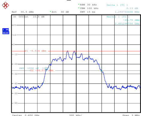
2DH1_Low 1.294MHz
