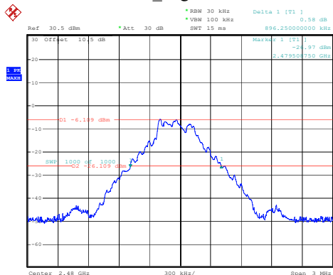
DH1_High 0.896MHz
