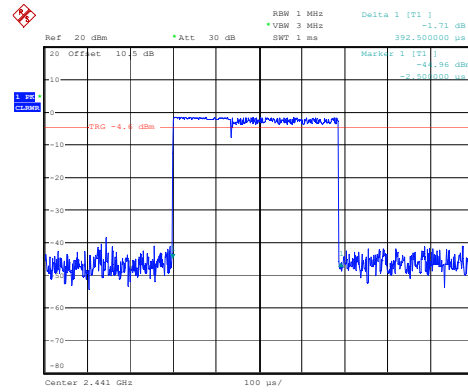
2DH1_Hopping 0.393ms
