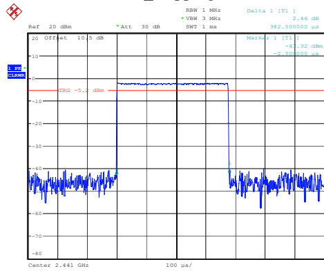
DH1_Hopping 0.383ms
