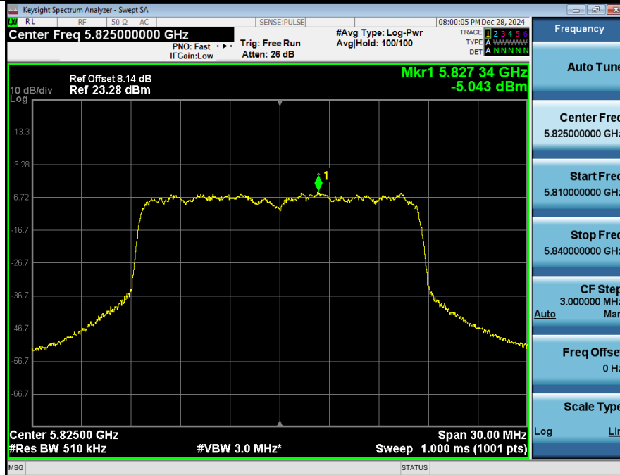
Power Spectral Density NVNT_ANT1_802_11n(HT20)_5825
