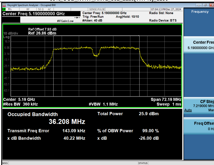
-26BW_NVNT_ANT1_802_11ac(VHT40)_5190
