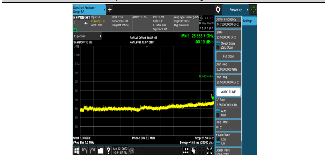
Band7-10MHz-QPSK-21100-1RB#0-Range5:3000~26500MHz
