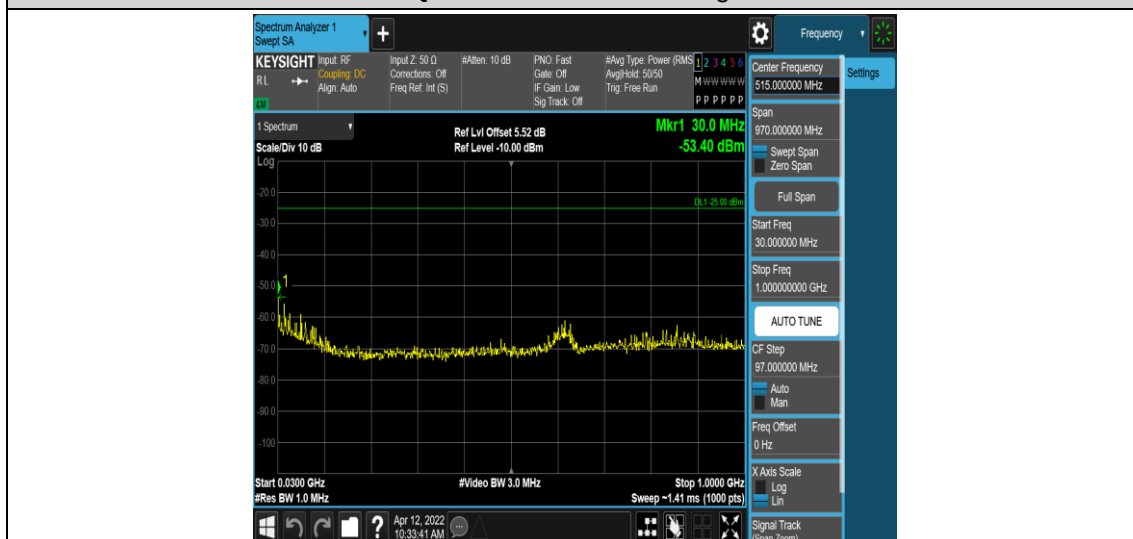
Band7-10MHz-QPSK-21400-1RB#0-Range3:30~1000MHz
