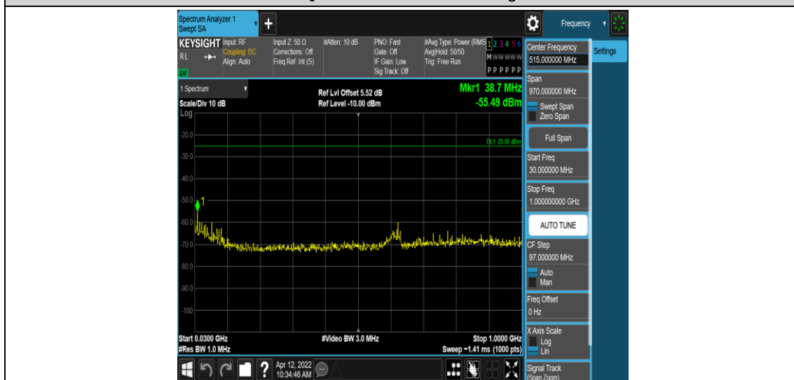
Band7-10MHz-16QAM-21400-1RB#0-Range3:30~1000MHz
